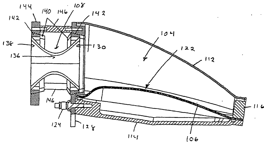
(SECTION B-B)
