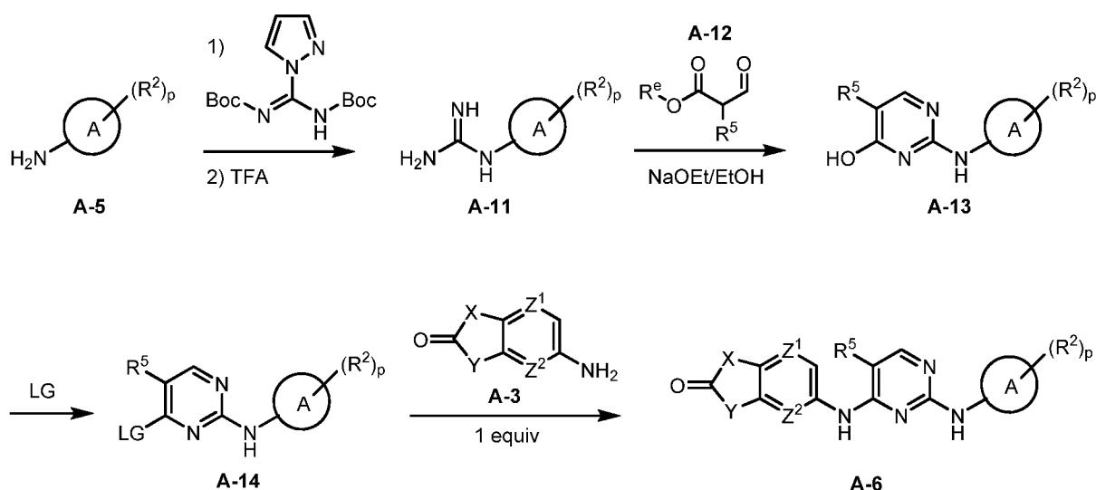
Scheme (II)
