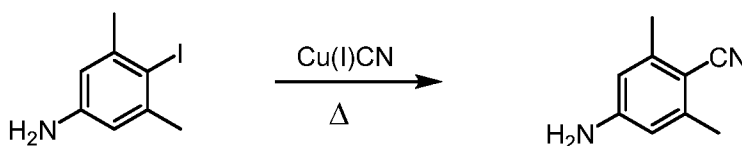
Scheme (VI)
