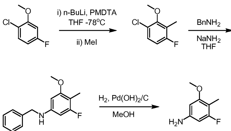
Scheme (IX)
