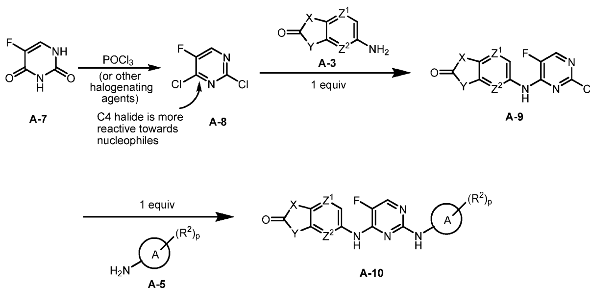
Scheme (Ia)
