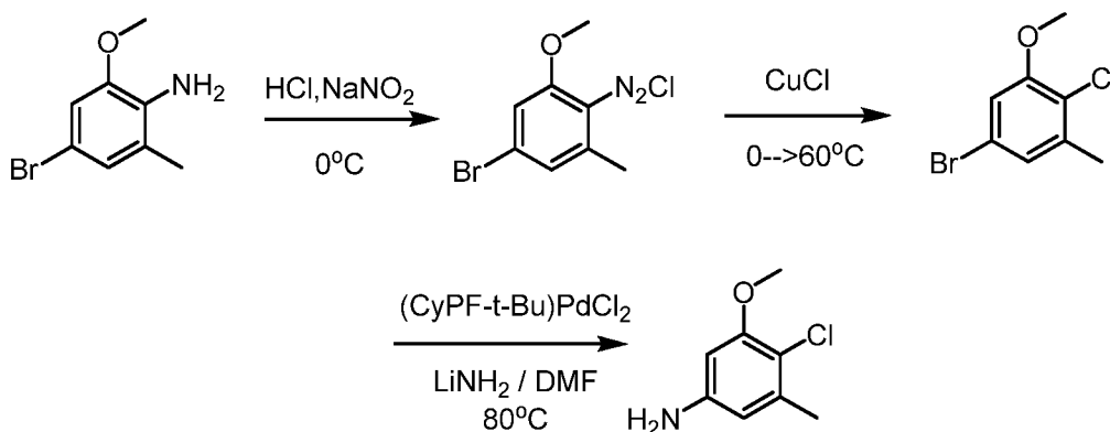
Scheme (VIII)
