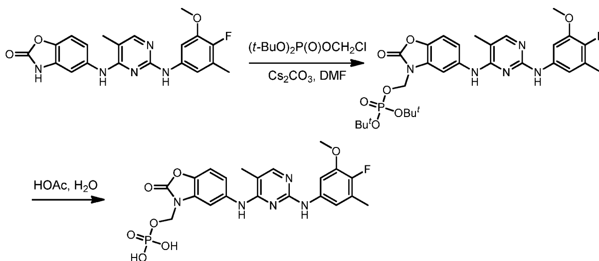
Scheme (XI)
