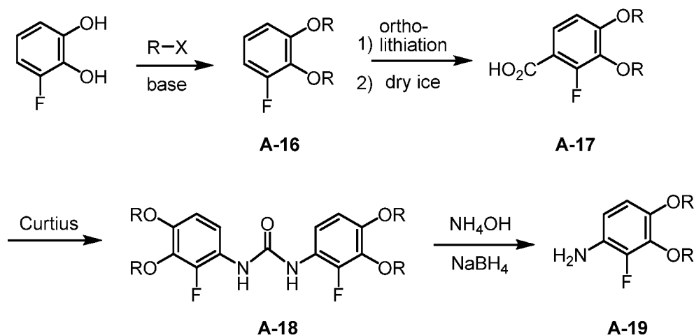
Scheme (III)
