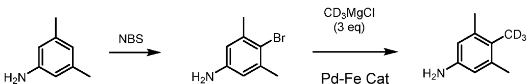
Scheme (V)
