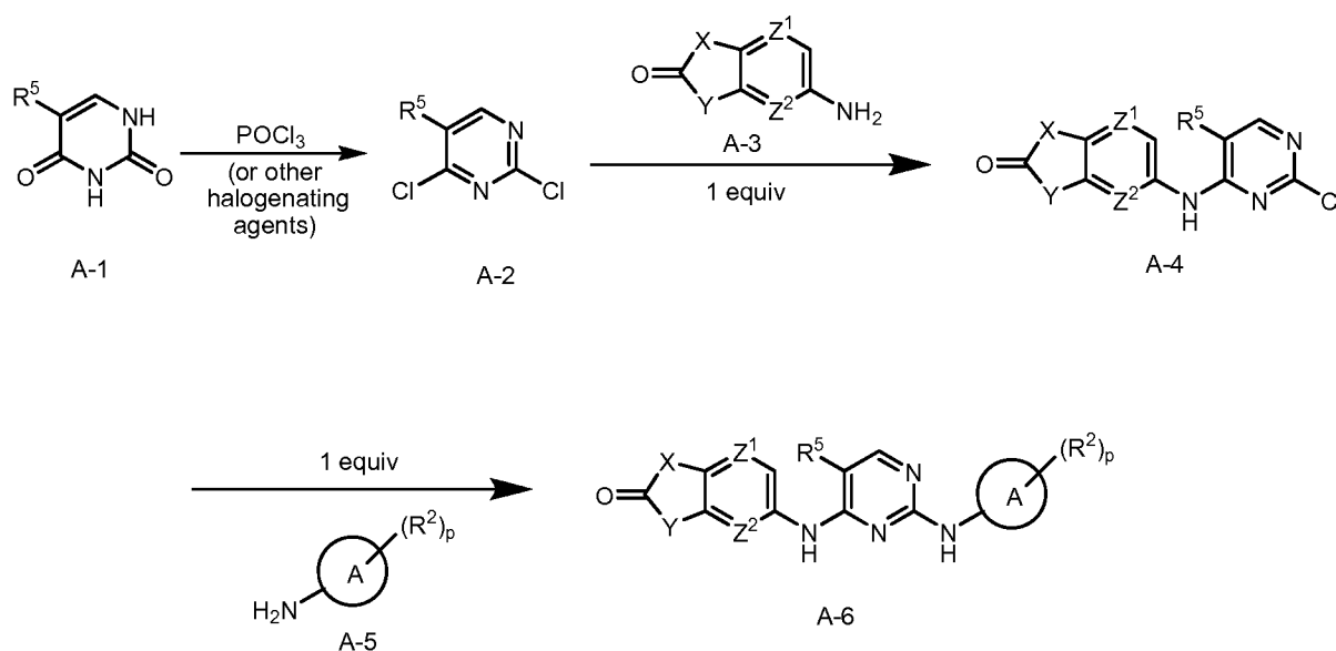
Scheme (I)
