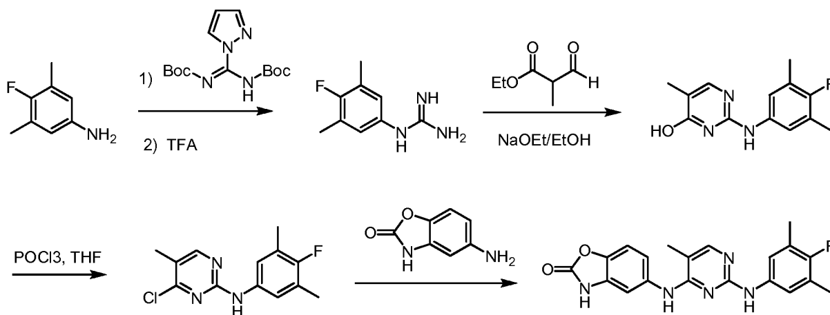
Scheme (X)
