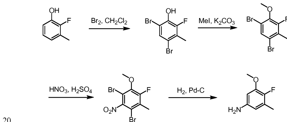
Scheme (VII)
