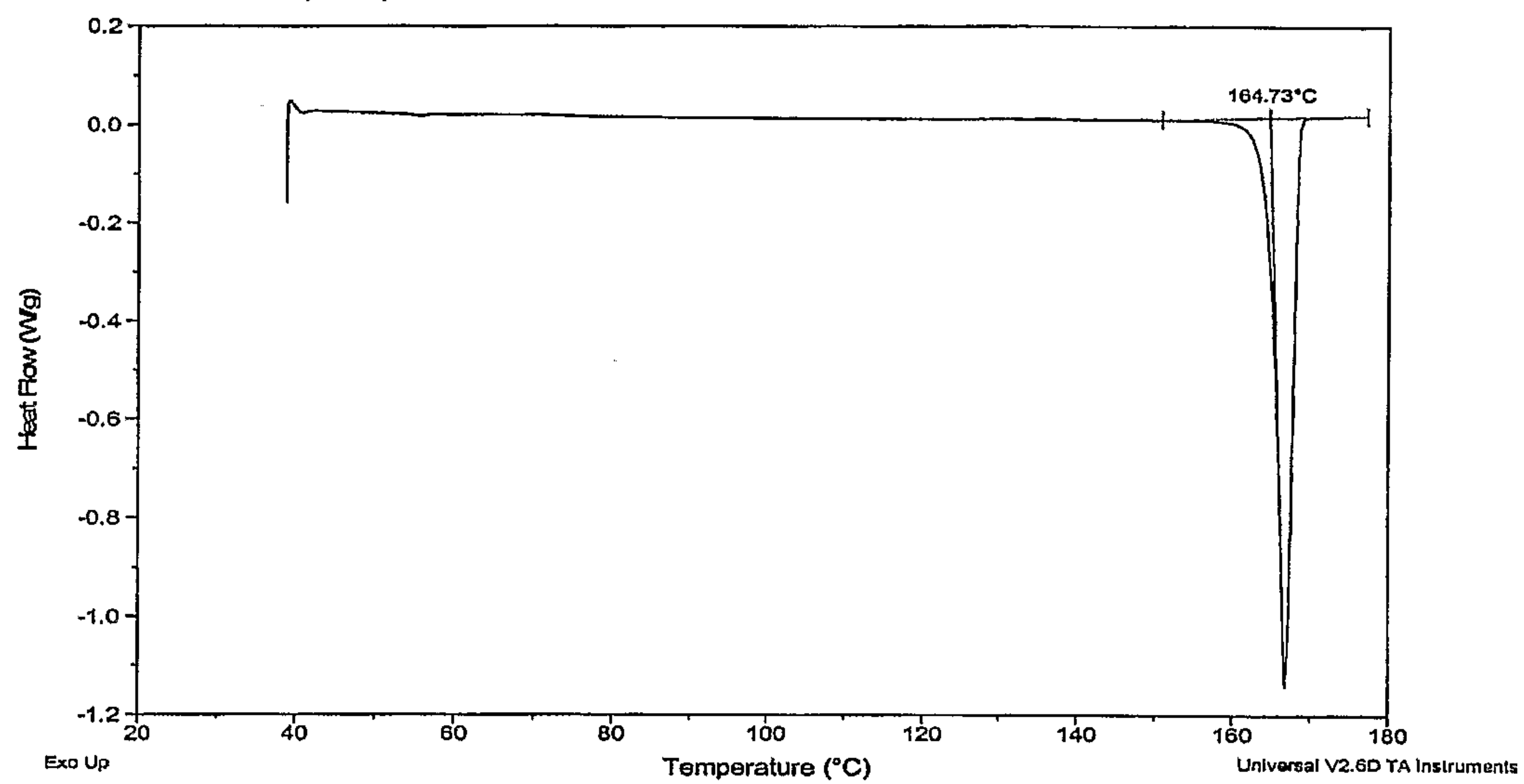
FIG. 13b: DSC trace for SMP-2-PRE. (Example 16)
