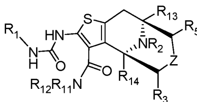
Formula (Ib).
