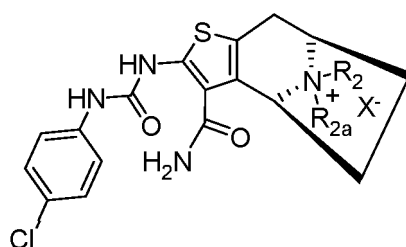
Formula (IIb'');
