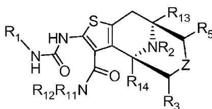
Formel (Ib).
