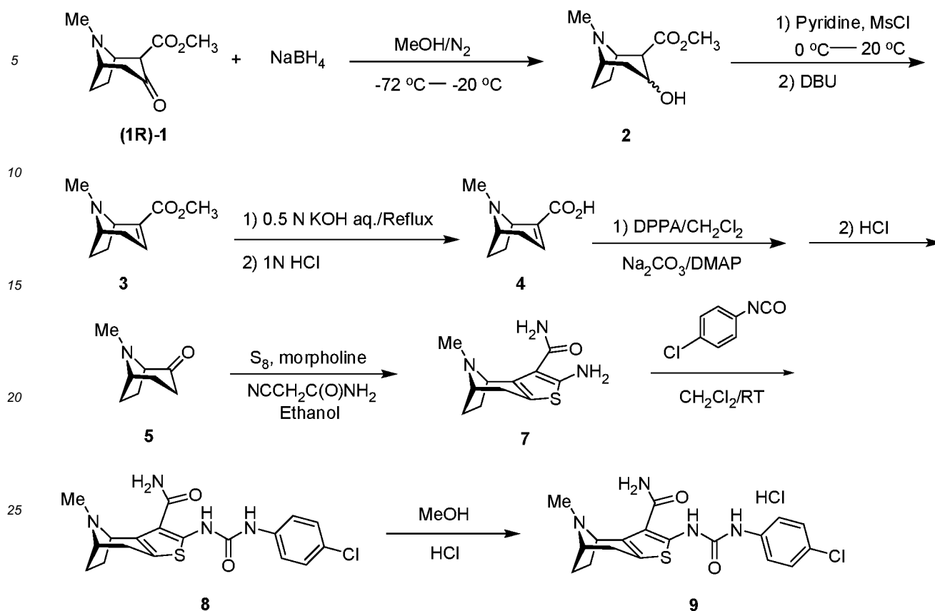
Scheme 2
