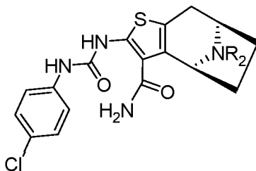
Formula (Ib'');
