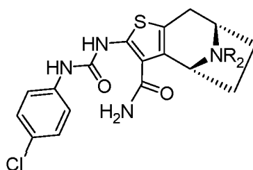
Formula (Ia'');
