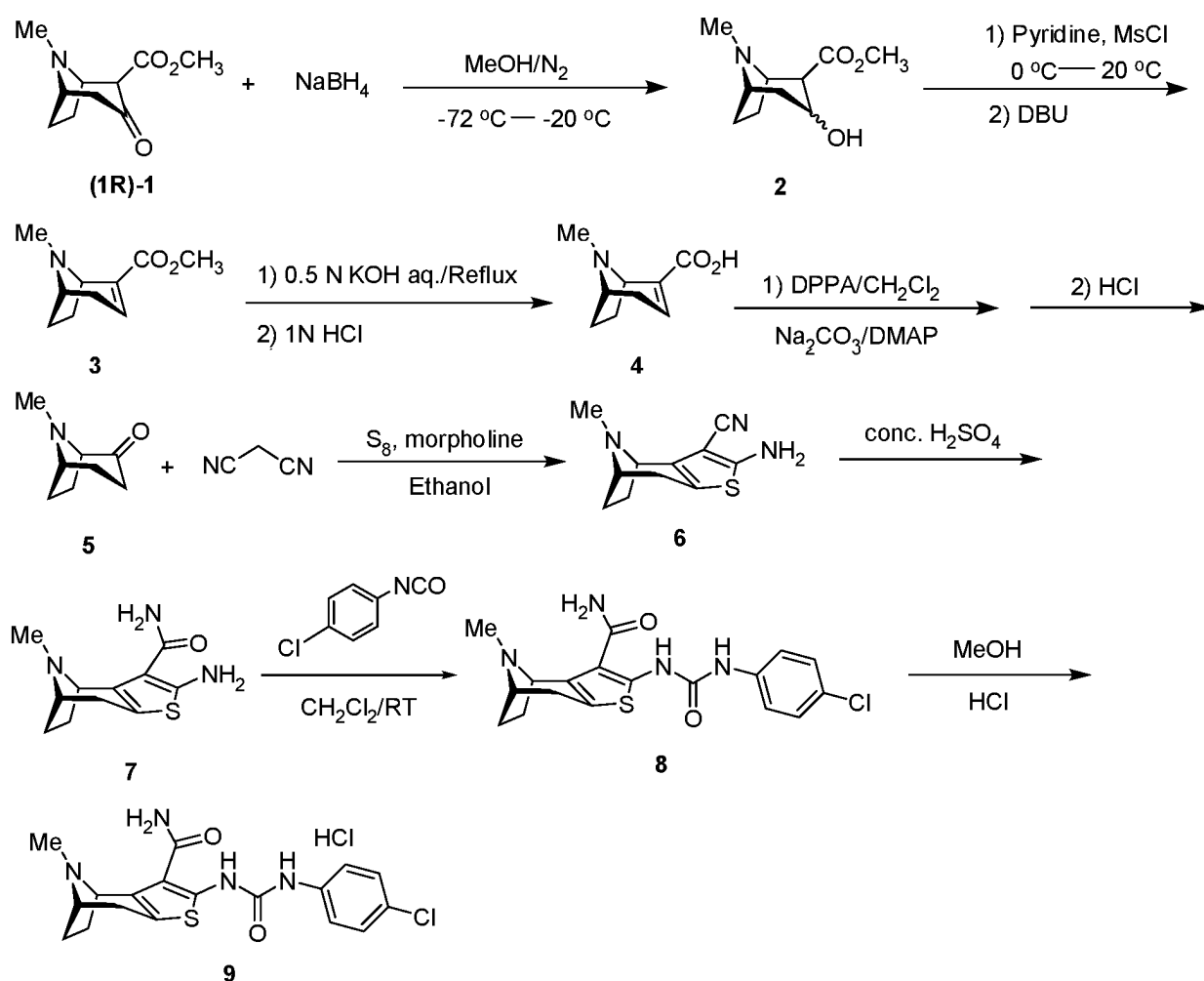
Scheme 1
