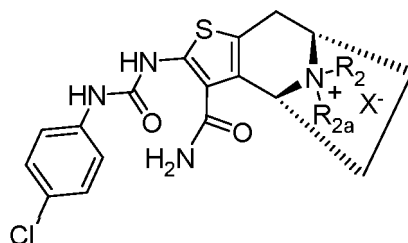
Formula (IIa'');
