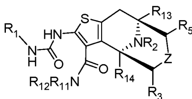
Formula (Ib);
