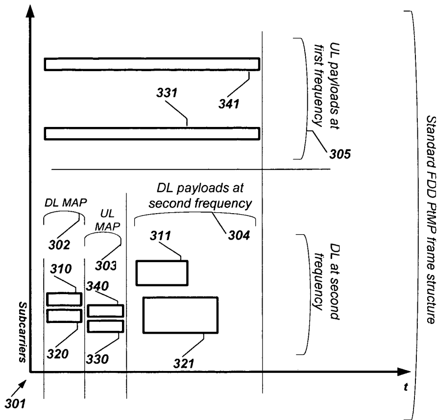
FIG. 4C - PRIOR ART
