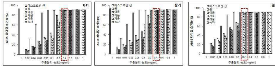
ABTS
