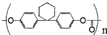
Structural Formula 1
