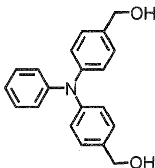
Compound 2
