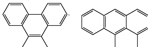
9,10-PhAn
