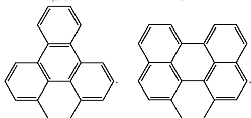
1,12-TriP
