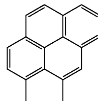
1,10-Pyr
