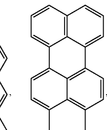
3,4-Per
