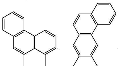
1,10-PhAn
