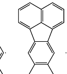
8,9-FlAn
