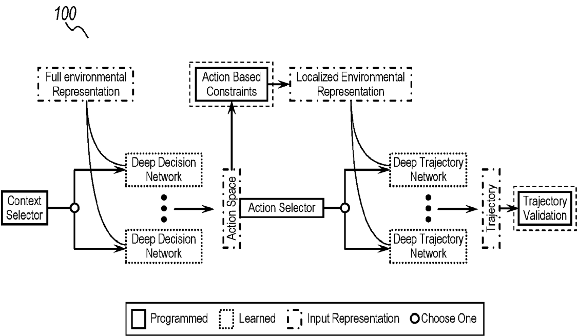
Architecture of Safety confined Hybrid Trajectory Generator
