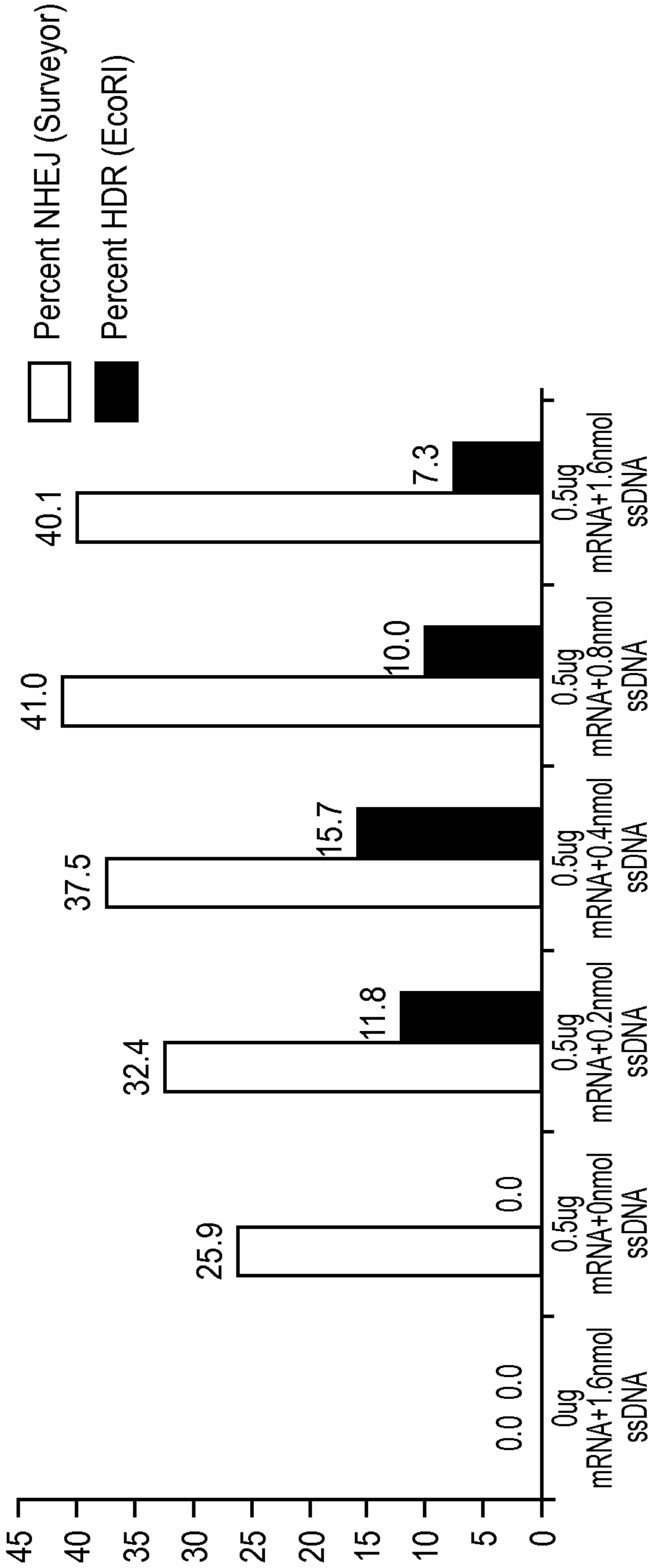
C313Y introduced into Ossabaw cells using TALENs and oligos
