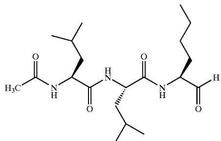
N-Acetyl-Leu-Leu-Nle-CHO
