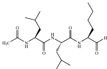
N-Acetyl-Leu-Leu-Nle-CHO
