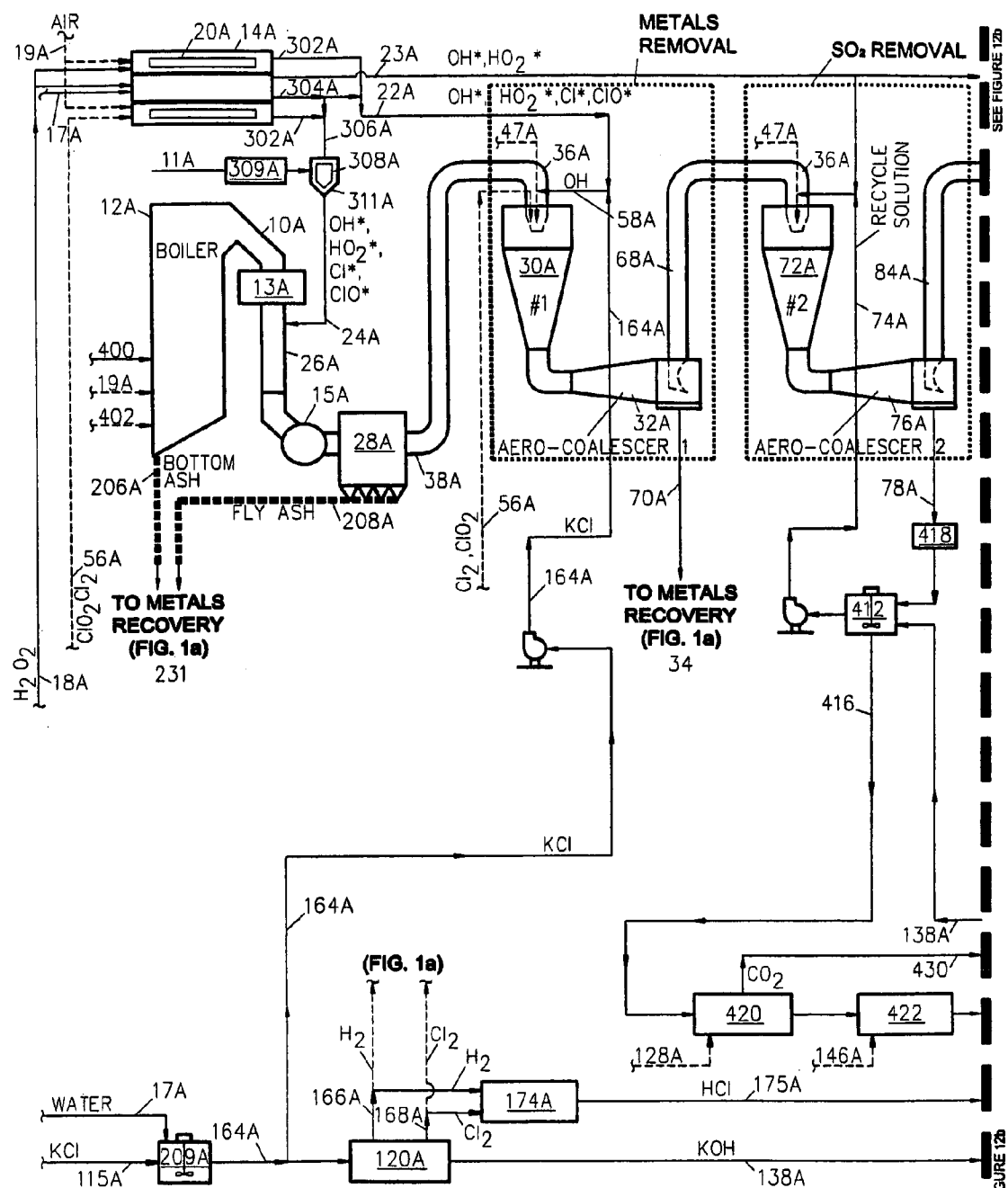
FIGURE 12a - PROCESS FOR MAXIMIZING CO2 RECOVERY & PRODUCTION
