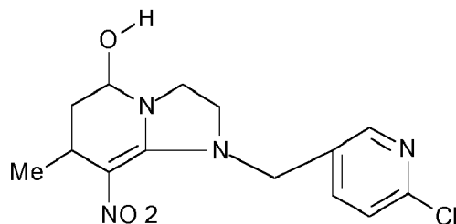
n) 1-((6-chloro-3-pyridinyl)methyl)-1,2,3,5,6,7-hexahydro-7-methyl-8-nitro-5-hydroxy-imidazo[1,2-a]pyridine
