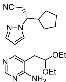
(Compound (I-2)),
