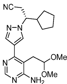
(Compound (I-1)),
