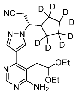
(Compound (I-2d)),
