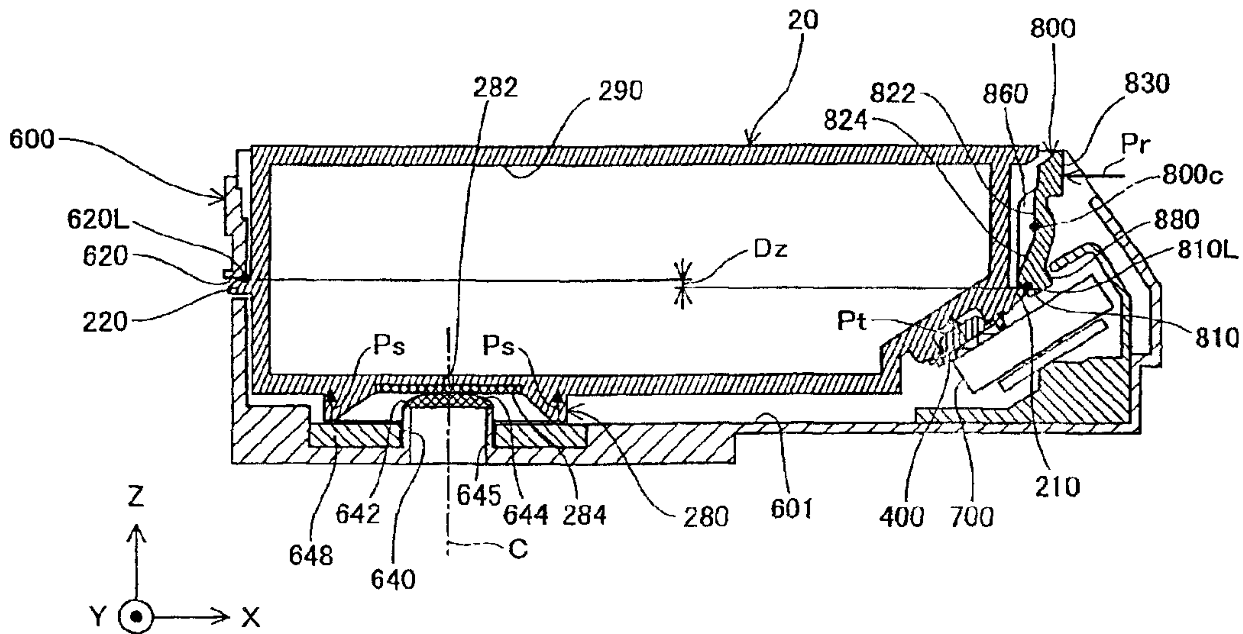
SECTION F5-F5
