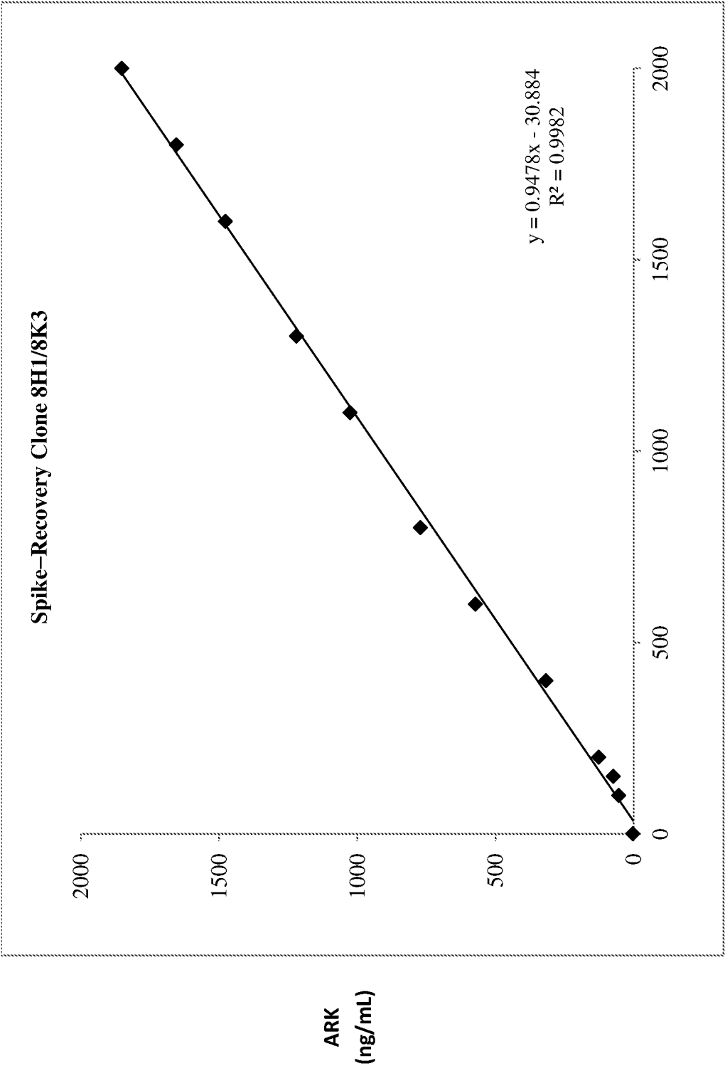
SDMA-Gly-Gly Dipeptide (ng/mL)
