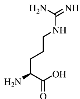
Arginine (ARG) FIG. 2 (RELATED ART)
