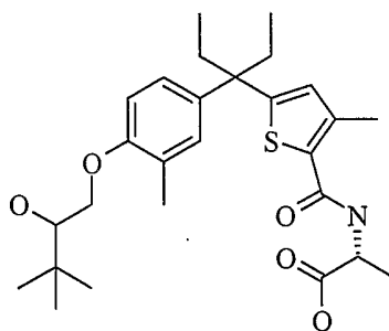
D -Epimer 1
