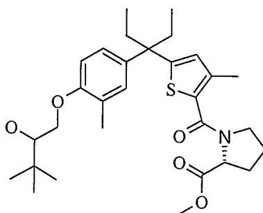
D -Epimer 2
