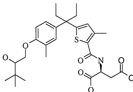
L -Epimer 2
