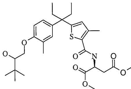
L -Epimer 2
