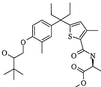
L -Epimer 1
