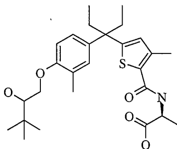
L -Epimer 1
