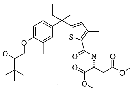
D -Epimer 2
