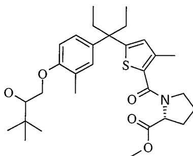
D -Epimer 1
