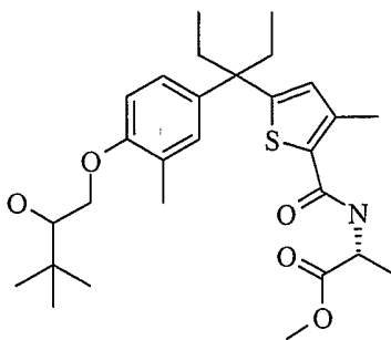
D -Epimer 1
