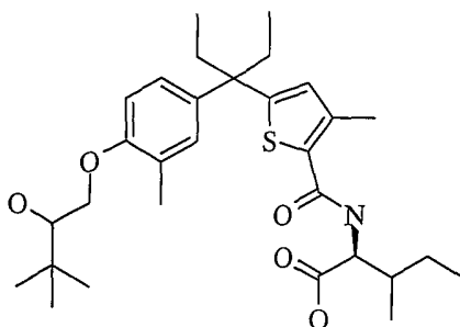
L -Epimer 1
