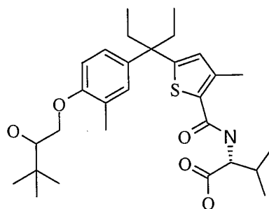
D -Epimer 2
