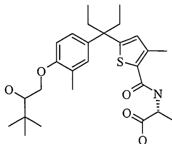
D -Epimer 2
