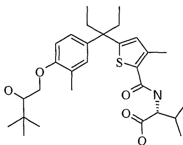
D -Epimer 1
