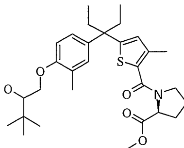
L -Epimer 1
