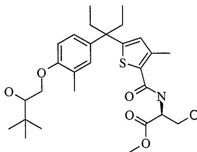
L -Epimer 2
