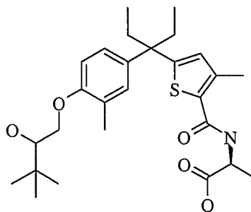
L -Epimer 2
