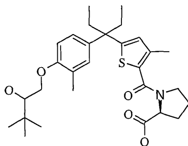
L -Epimer 2
