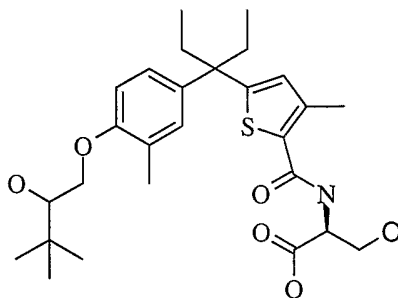
L -Epimer 2
