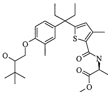
L -Epimer-2
