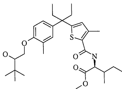
L -Epimer 1
