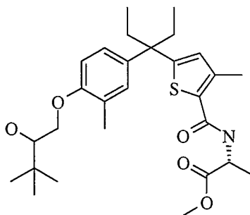
15 D -Epimer 2
