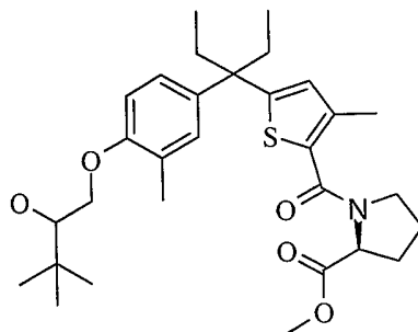
L -Epimer 2
