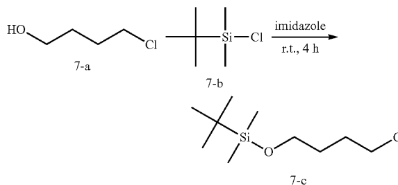
Scheme 7: Synthesis of tert-butyl(4-chlorobutoxy)dimethylsilane (7-c)
