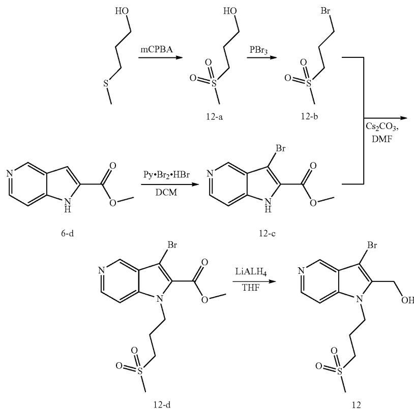
Scheme 12: synthesis of (3-bromo-1-(3-methylsulfonyl)propyl)-1H-pyrrolo[3,2-c]pyridin-2-yl)methanol 12
