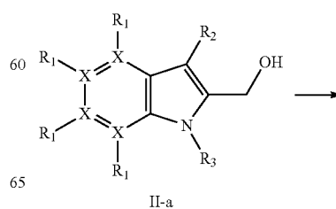
Scheme 3: General synthesis of II-b and II-c type compounds
