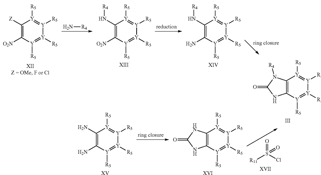
Scheme 4: General synthesis of III type compounds
