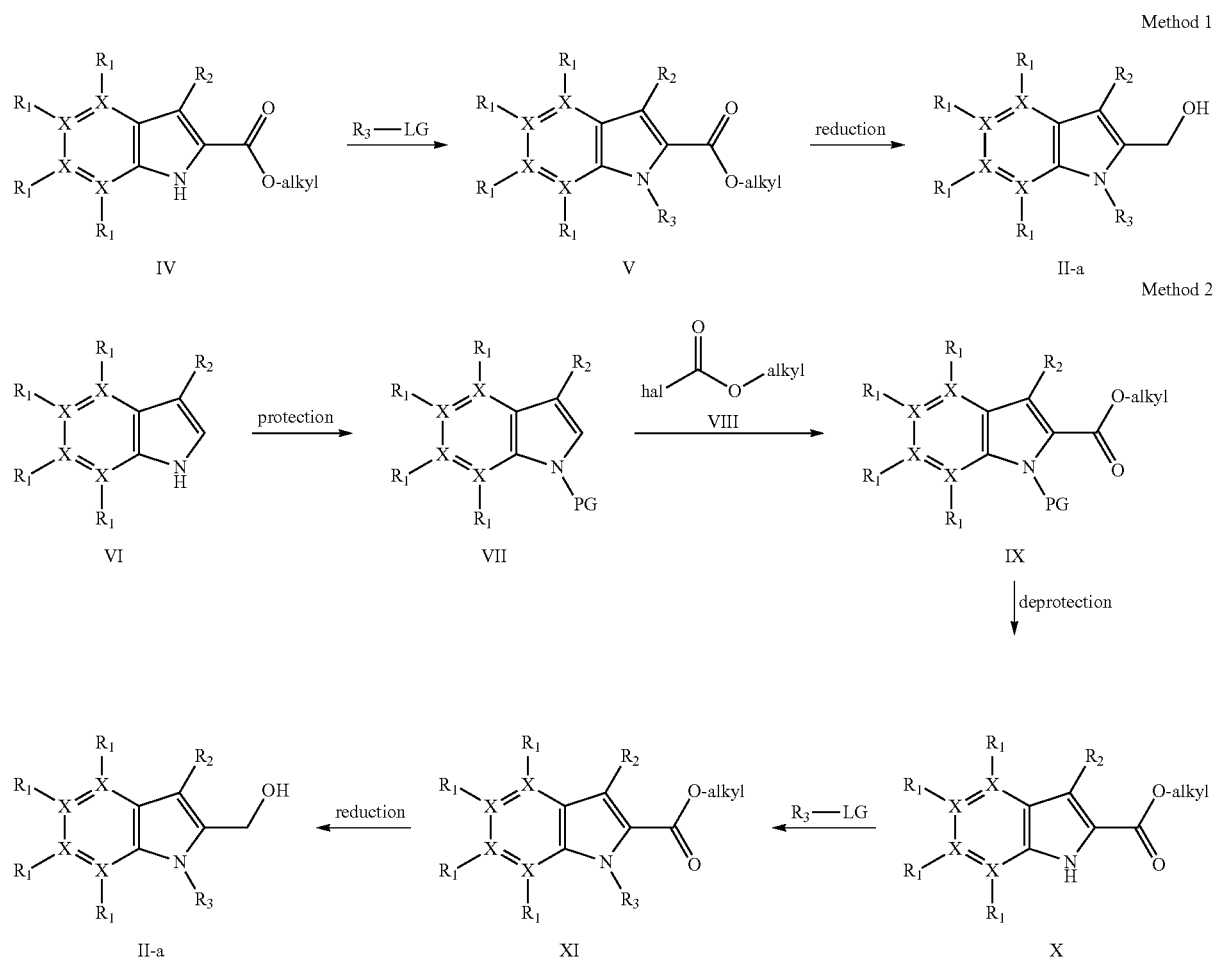
Scheme 2: General synthesis of II-a type compounds
