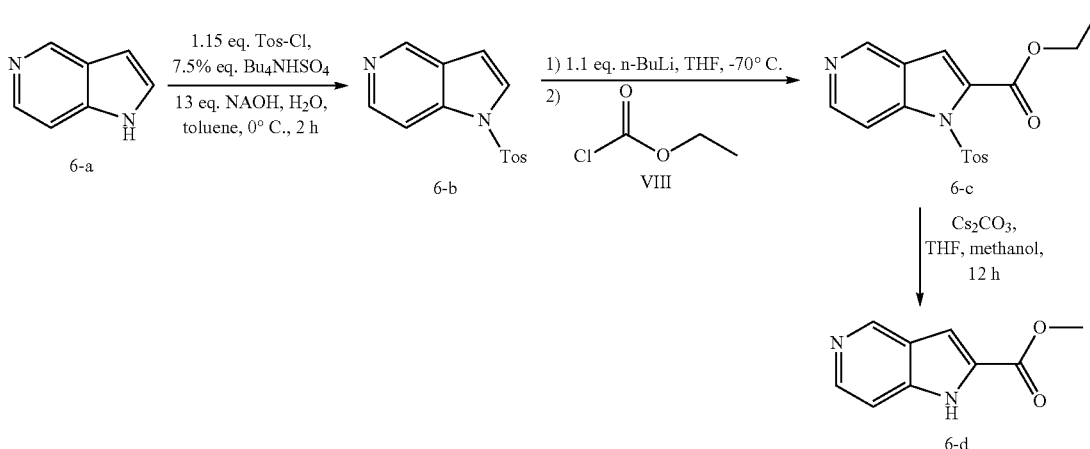
Scheme 6: Synthesis of methyl 1H-pyrrolo[3,2-c]pyridine-2-carboxylate (6-d)
