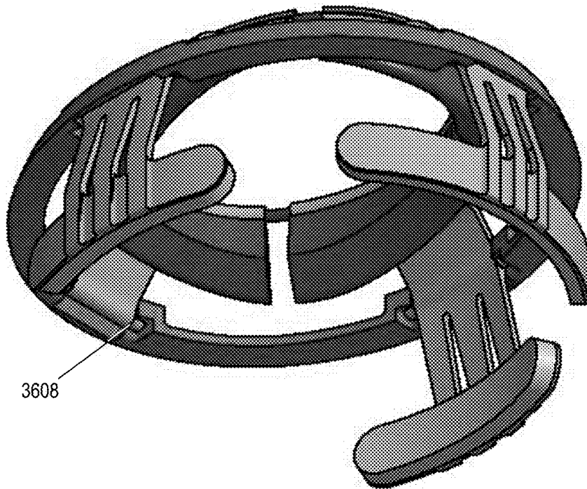
(PERSPECTIVE) 3600 FIG. 36B
