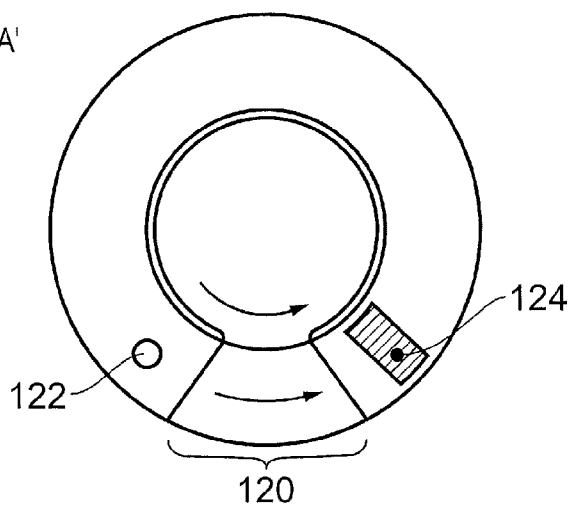
FIG. 2 (Prior Art)
