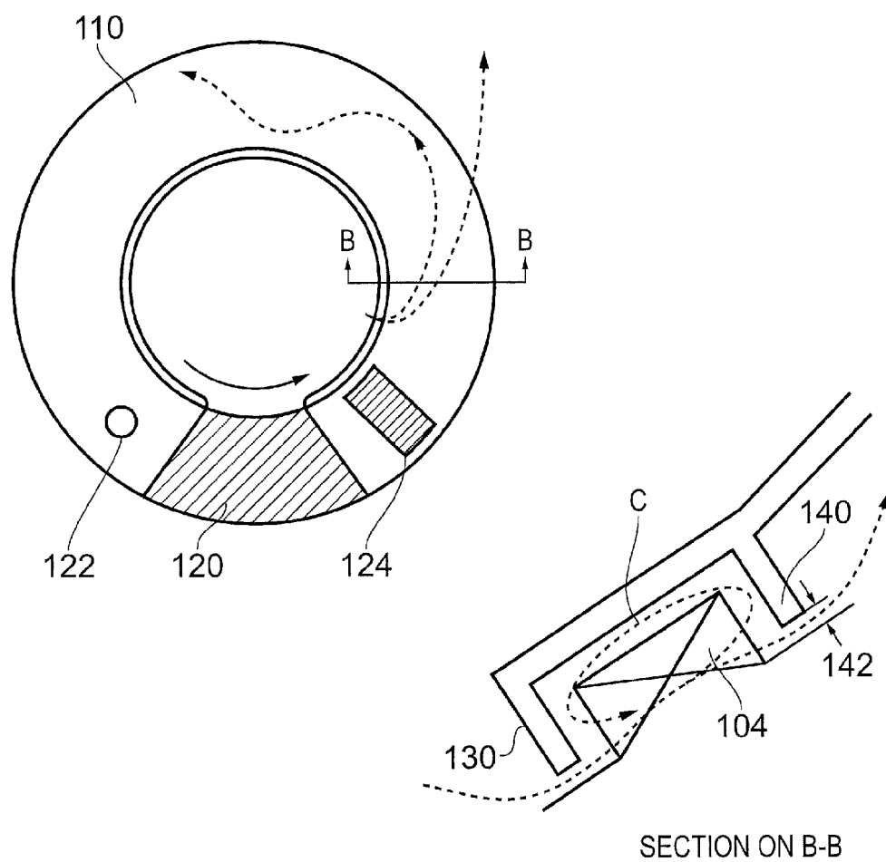
FIG. 3 (Prior Art)
