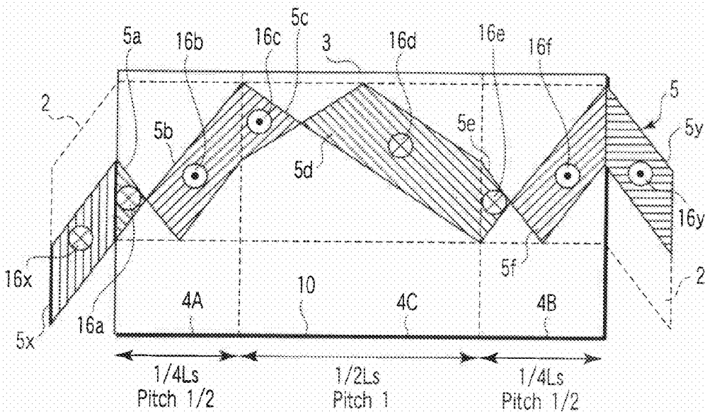
FIG. 27 (PRIOR ART)
