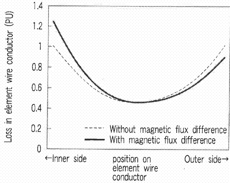
FIG. 31 (PRIOR ART)
