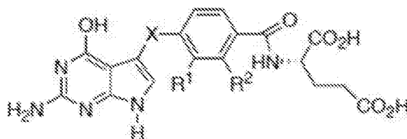
FIG. 1Q Exemplary Pemetrexed Derivatives
