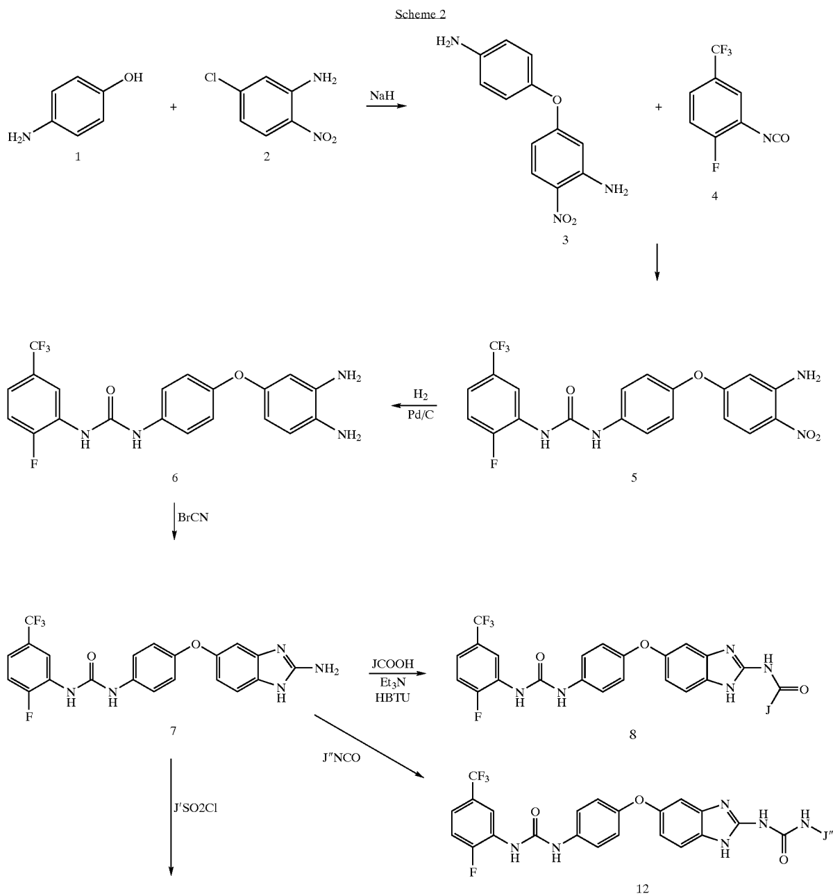
Scheme 2
