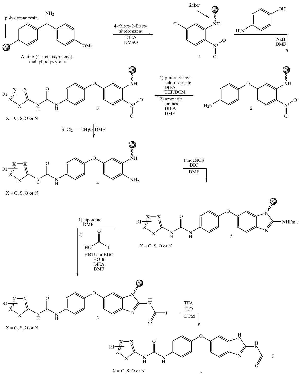
Scheme 13
