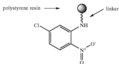
Intermediate 14A
