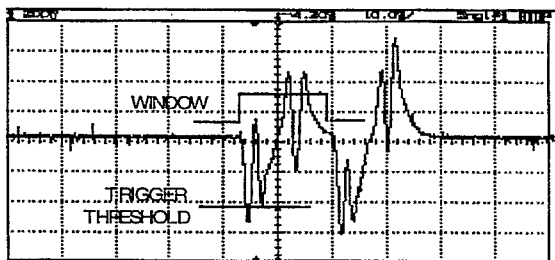
Fig. 4 (d). Signature of two successive beads (horizontal - time 10msec/div) (vertical - voltage 10V/div)
