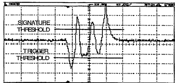
Fig. 4 (c). Signature of a single bead (horizontal - time 10msec/div) (vertical - voltage 10V/div)
