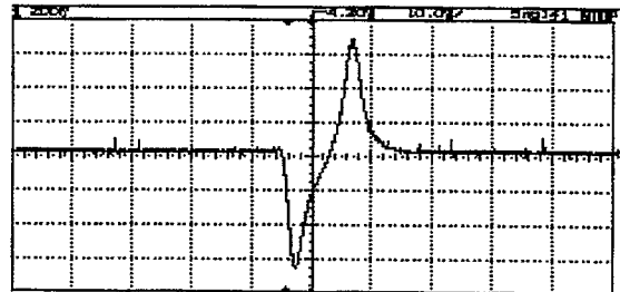
Fig. 4 (b). Signature of a bubble (horizontal - time 10msec/div) (vertical - voltage 10V/div)
