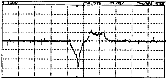
Fig. 4(a). Signature of a bead fragment (horizontal - time 10msec/div) (vertical - voltage 10V/div)
