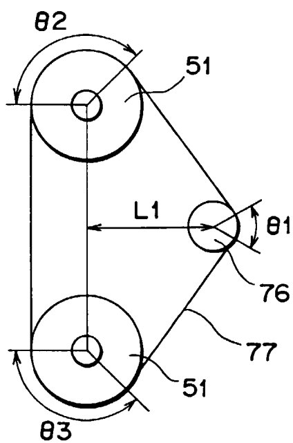
FIG. 3 (PRIOR ART)
