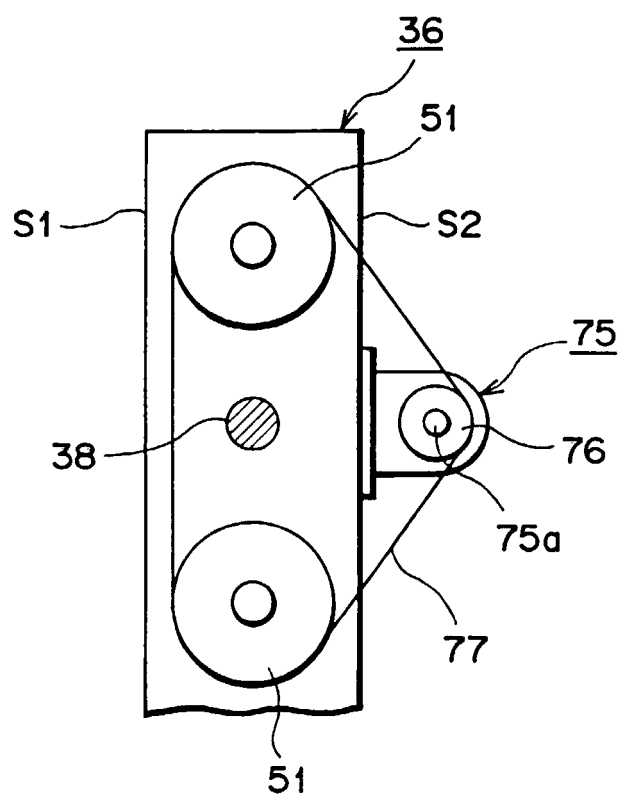
FIG. 2 (PRIOR ART)
