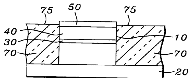
FIG. 3c - Prior Art
