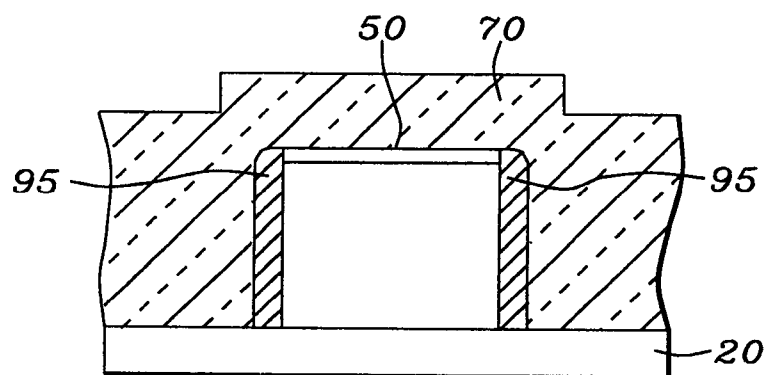
FIG. 4c - Prior Art
