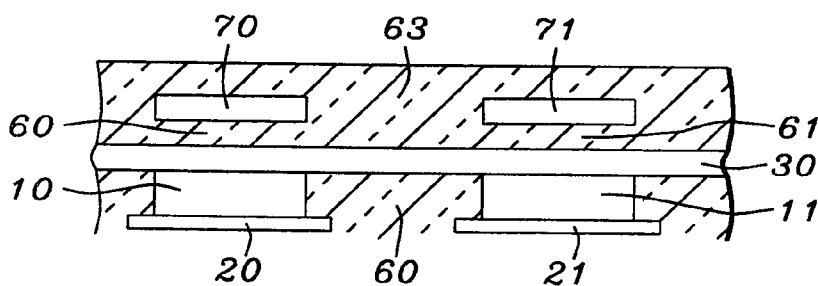
FIG. 2 - Prior Art
