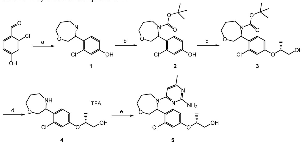
Scheme 1: Synthesis of Compound C-60
