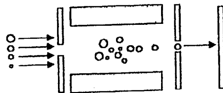
Simultaneous operations: Accumulation + Selective Ejection/Ion Landing
