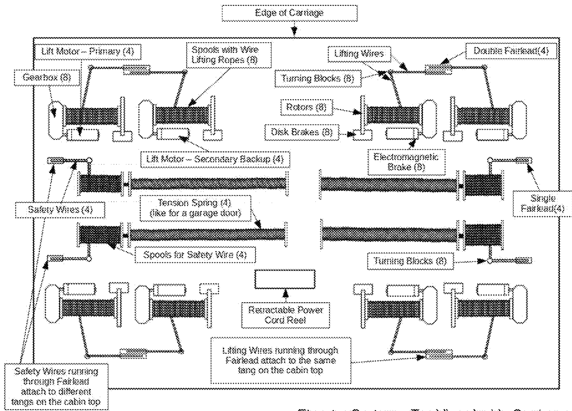
Elevator System -- Top View, Inside Carriage
