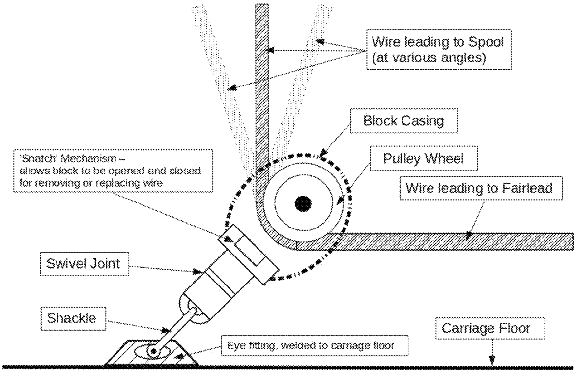
Turning Block - 'Snatch' Type
