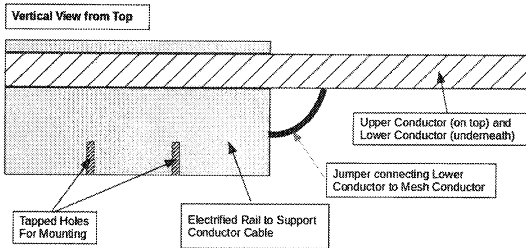
Detail of Jumper Connecting Lower Conductor to Mesh Conductor
