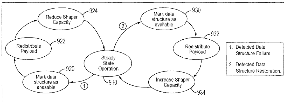
Link Aggregation Payload Redistribution State Diagram
