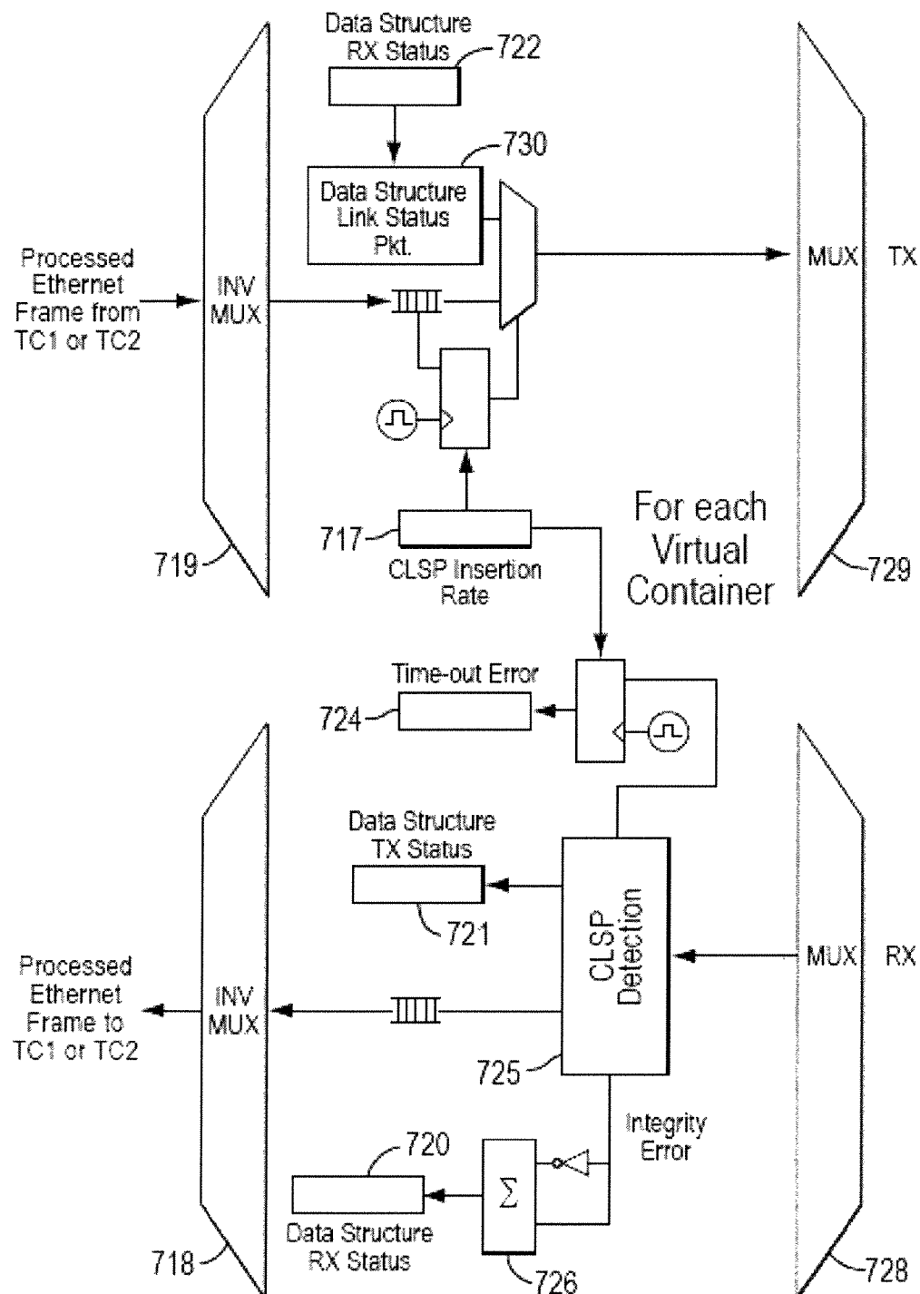
Engine for RCDF for data stream
