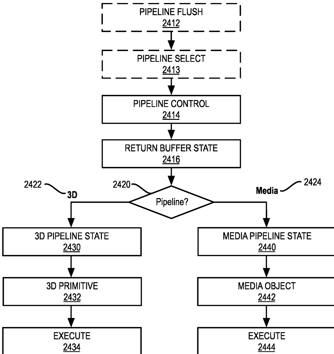
GRAPHICS PROCESSOR COMMAND SEQUENCE 2410
