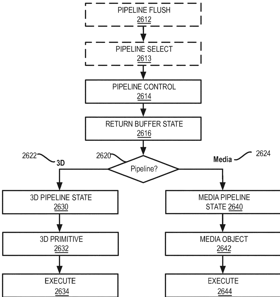
FIG. 26B GRAPHICS PROCESSOR COMMAND SEQUENCE 2610
