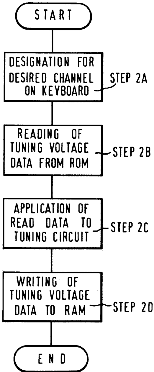
FIG. 2. (PRIOR ART)
