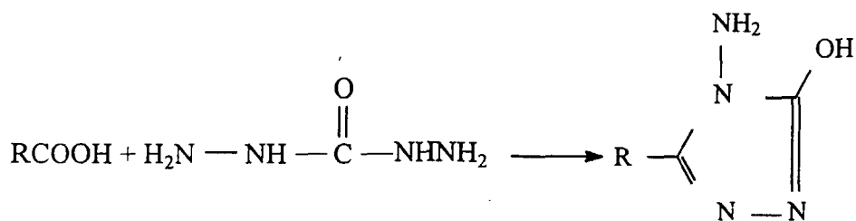
3-hydroxy-4-amino-triazole
