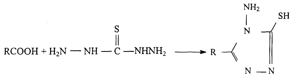
3-mercapto-4-amino-triazole
