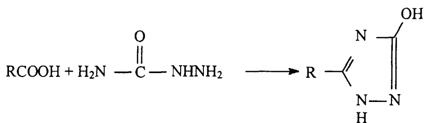
3-hydroxytriazole
