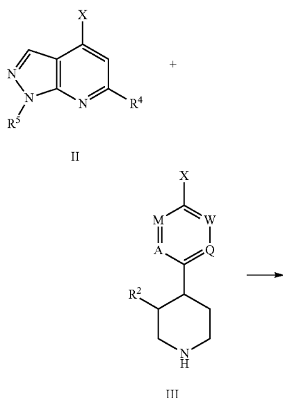
Scheme 1
