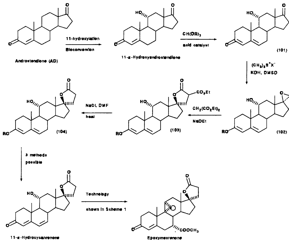
Scheme 7
