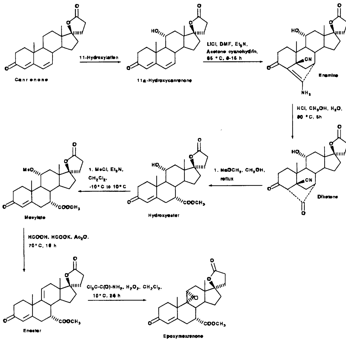
Scheme 2
