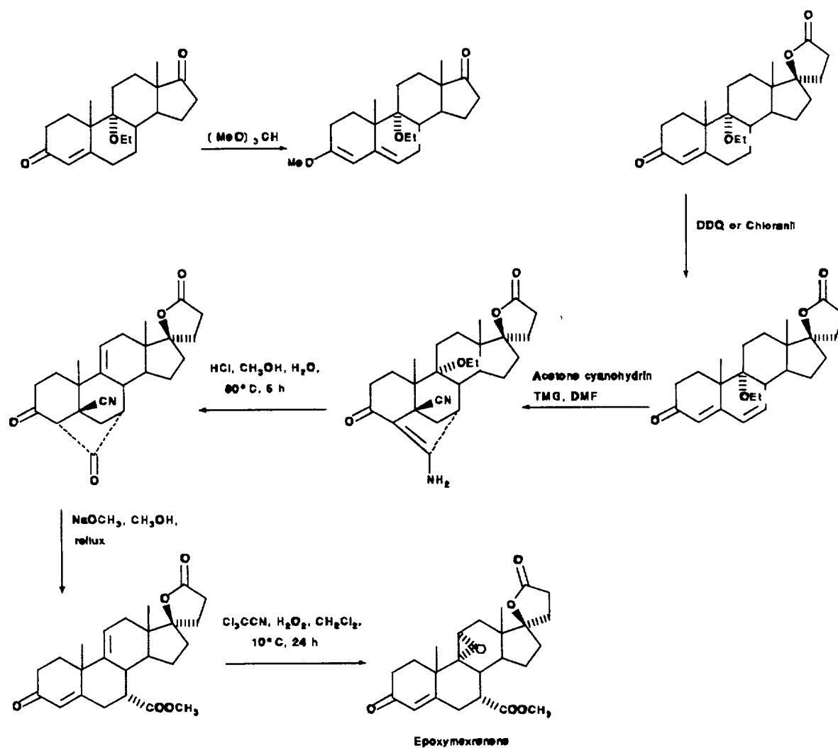
Scheme 6
