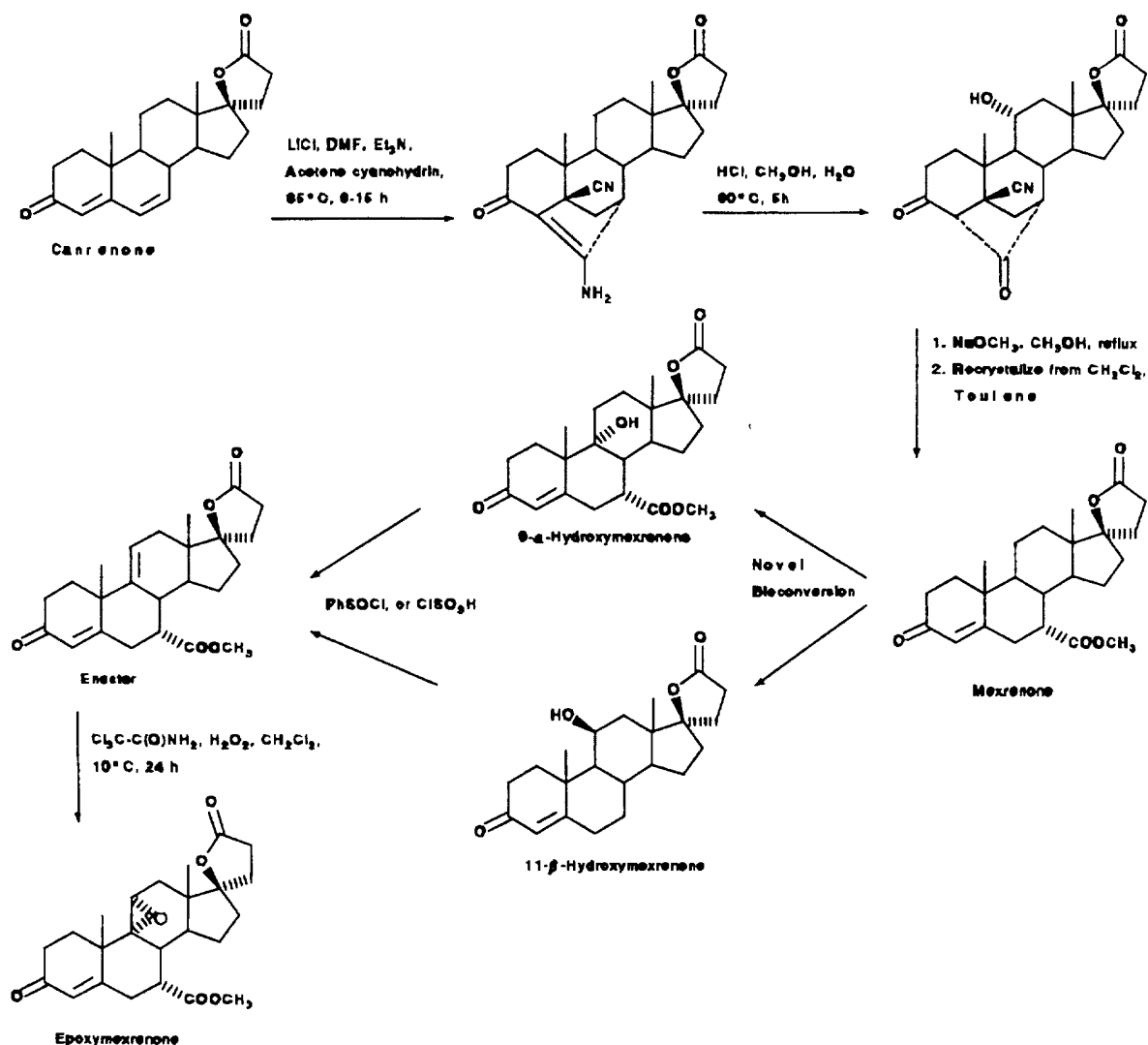
Scheme 3
