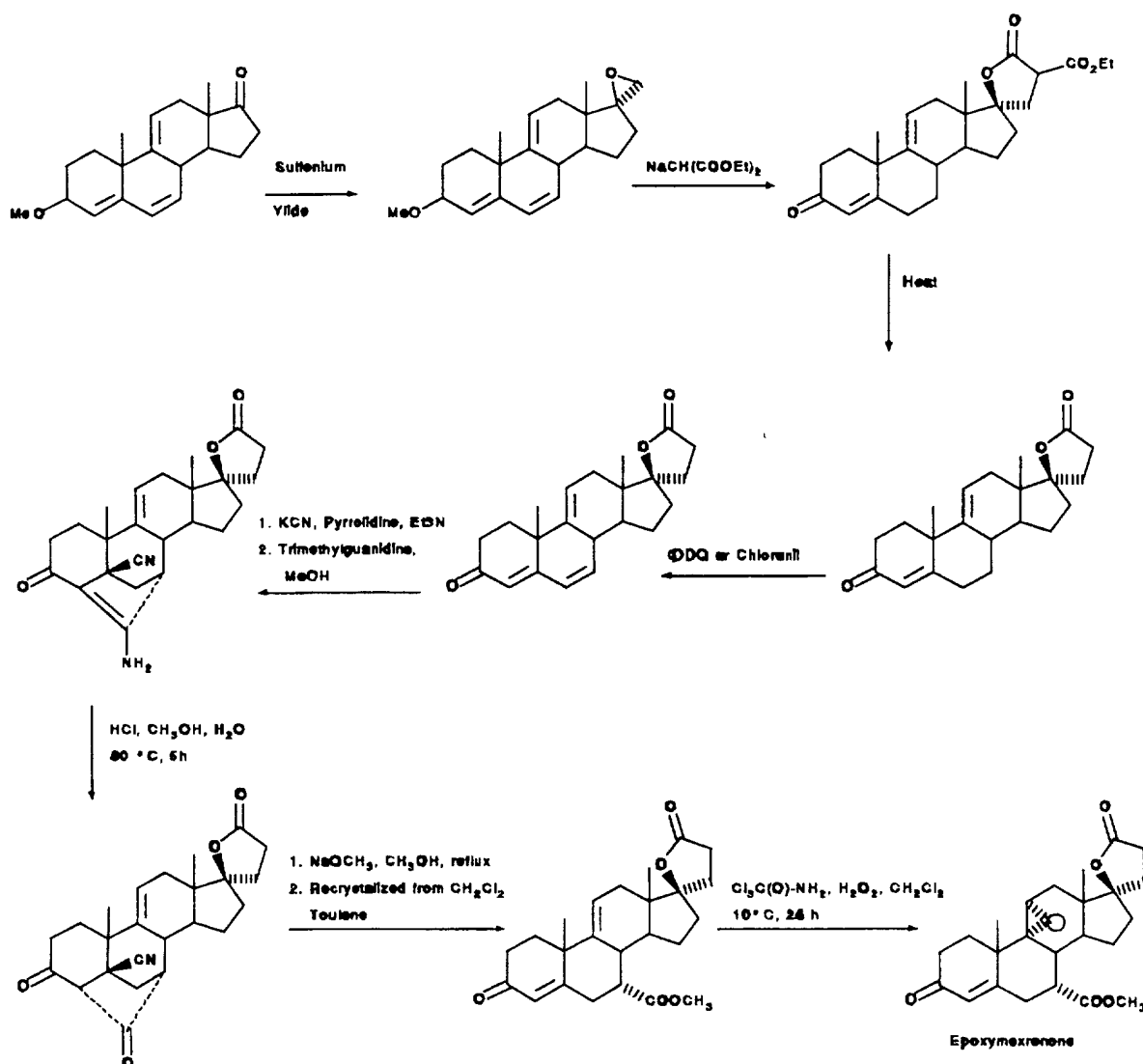
Scheme 4
