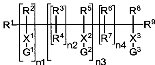
Formula I
