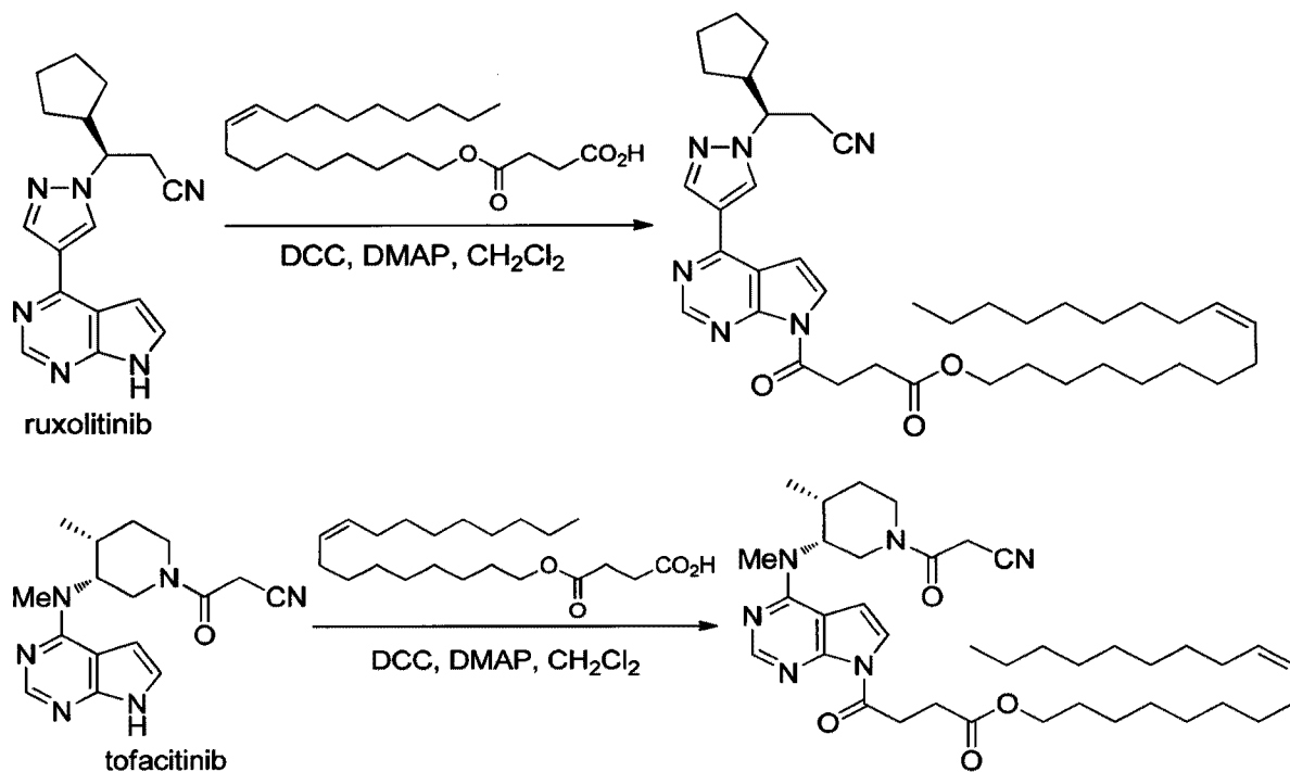
SCHEME 29. Scheme for synthesis of LDO1-RXN and LDO1-TFN
