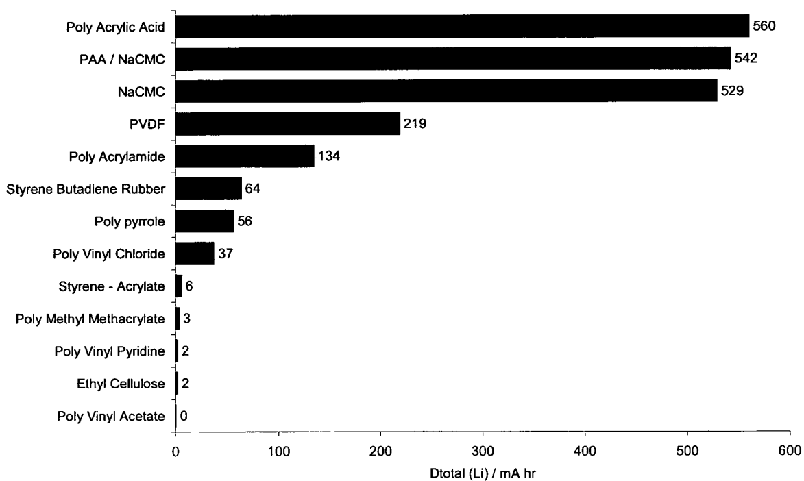
Figure 3. Total Delithiation Capacity Over One Hundred Cycles
