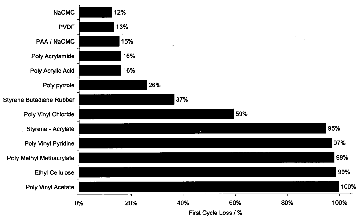
Figure 2. Comparison of first cycle losses with different binders
