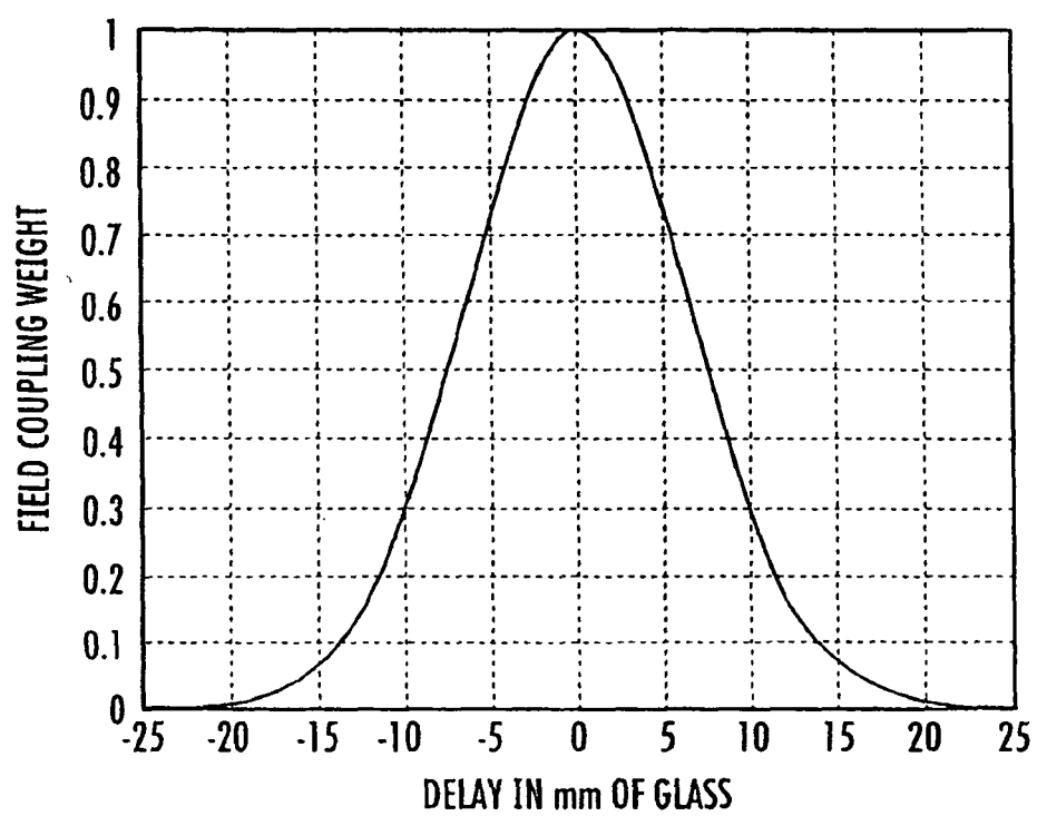
IMPULSE RESPONSE OF 10 GHz BANDPASS GAUSSIAN FILTER
