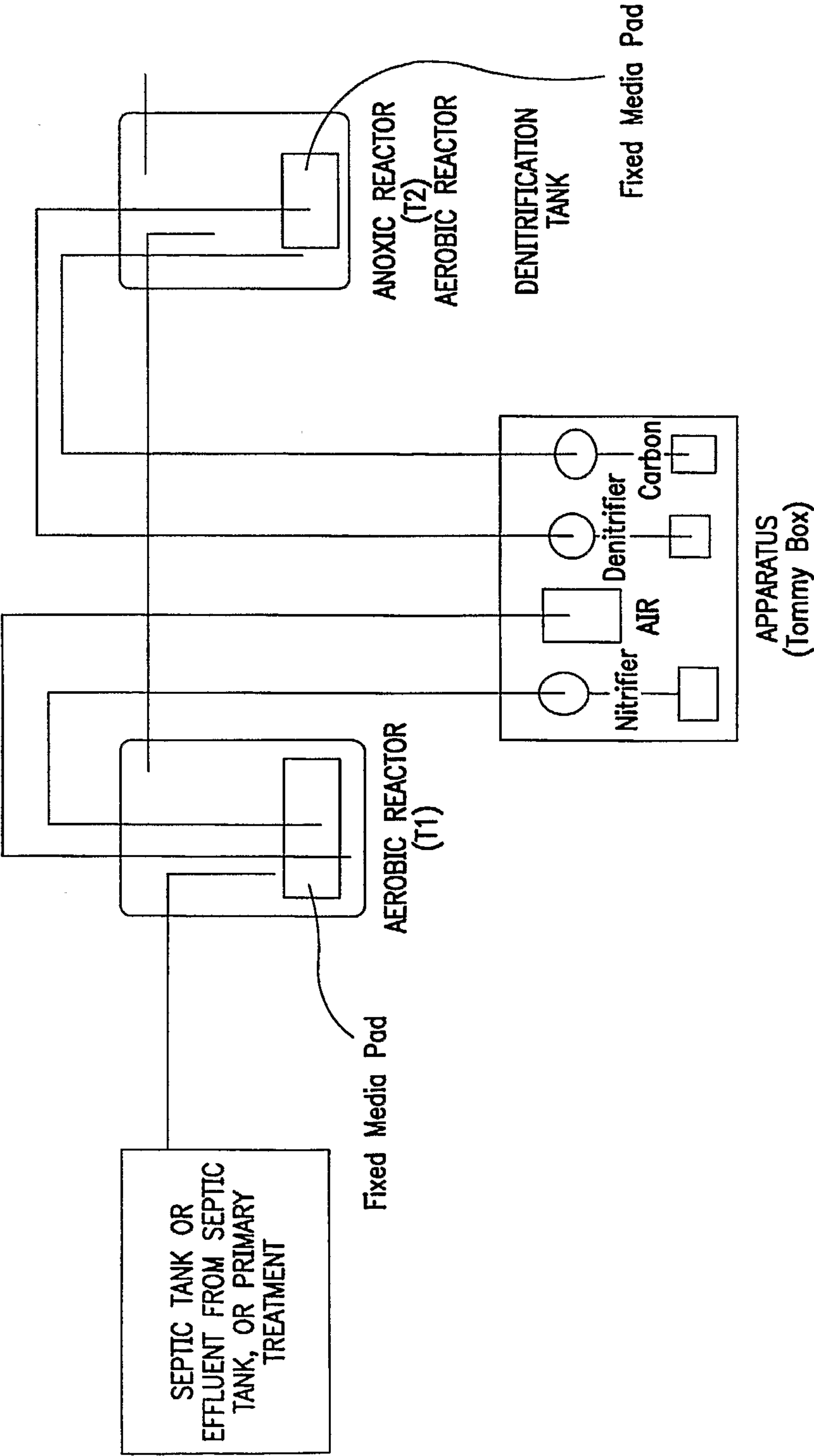
Layout for Apparatus shown for 1 liter Reactors with Fixed Media in the Oxic and Anoxic Reactors
