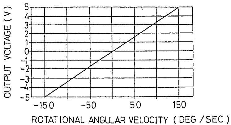
OUTPUT VOLTAGE CHARACTERISTICS (ERECT)
