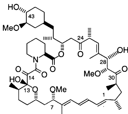
15 28-epirapamycin
