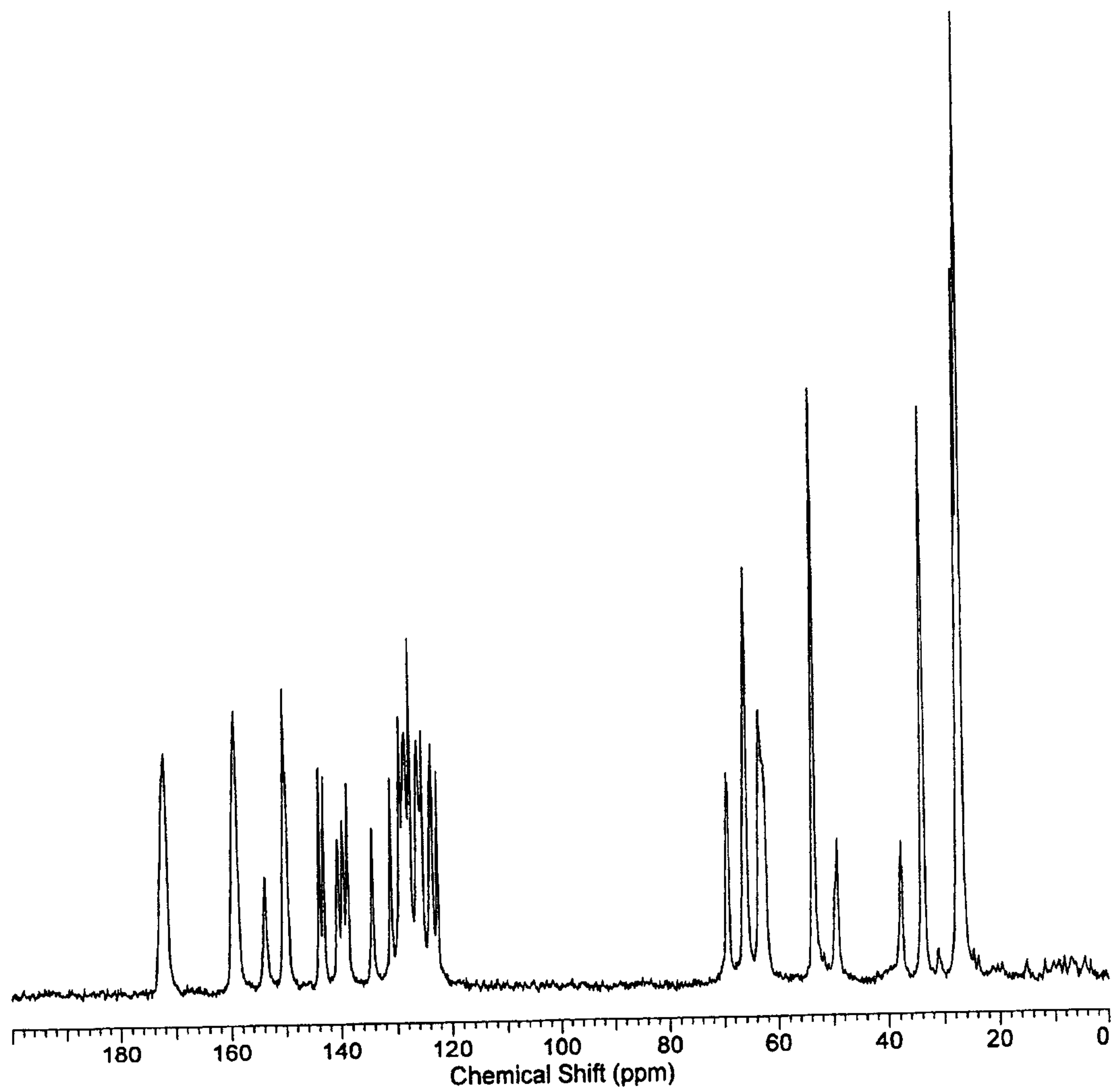
Carbon-13 SSNMR of FORM A
