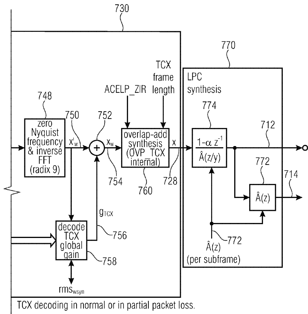
Block diagram of the TCX decoder FIG 7B
