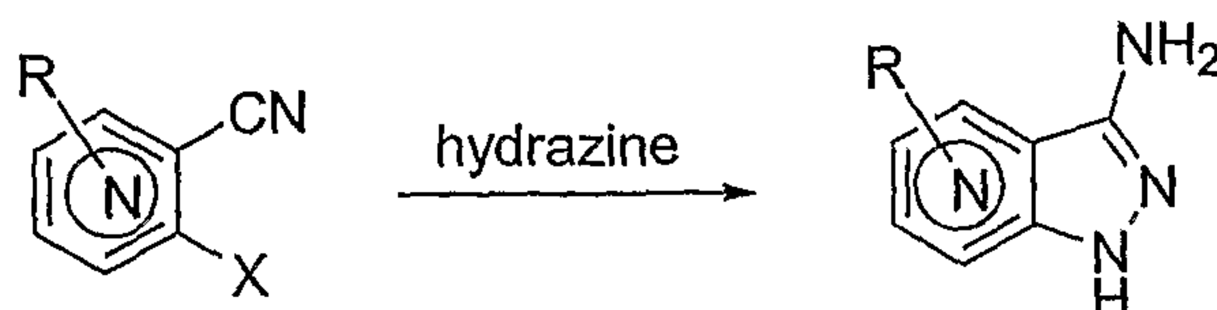
Scheme 1C
