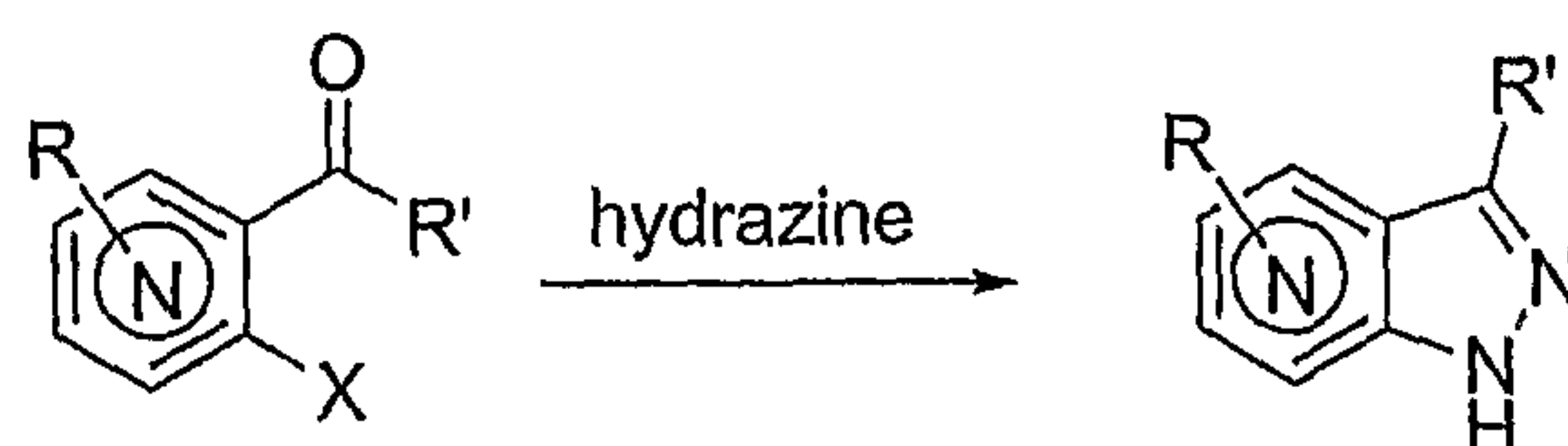
Scheme 1B
