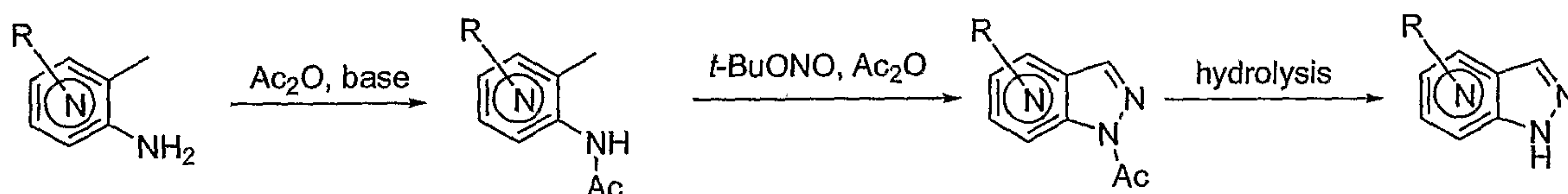
Scheme 1D
