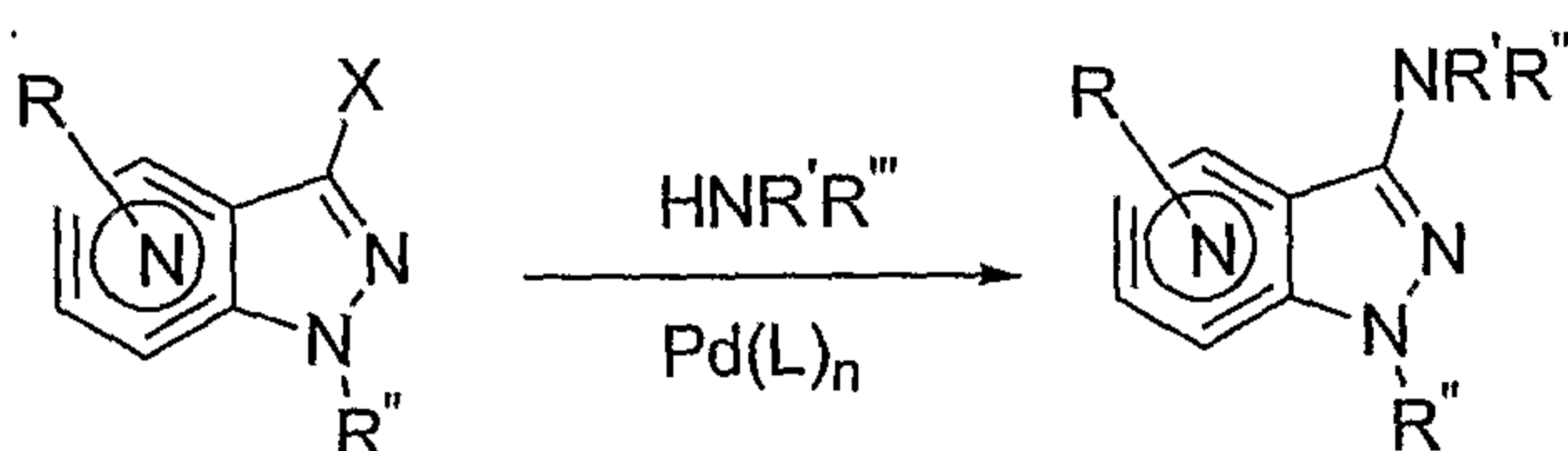
Scheme 1H
