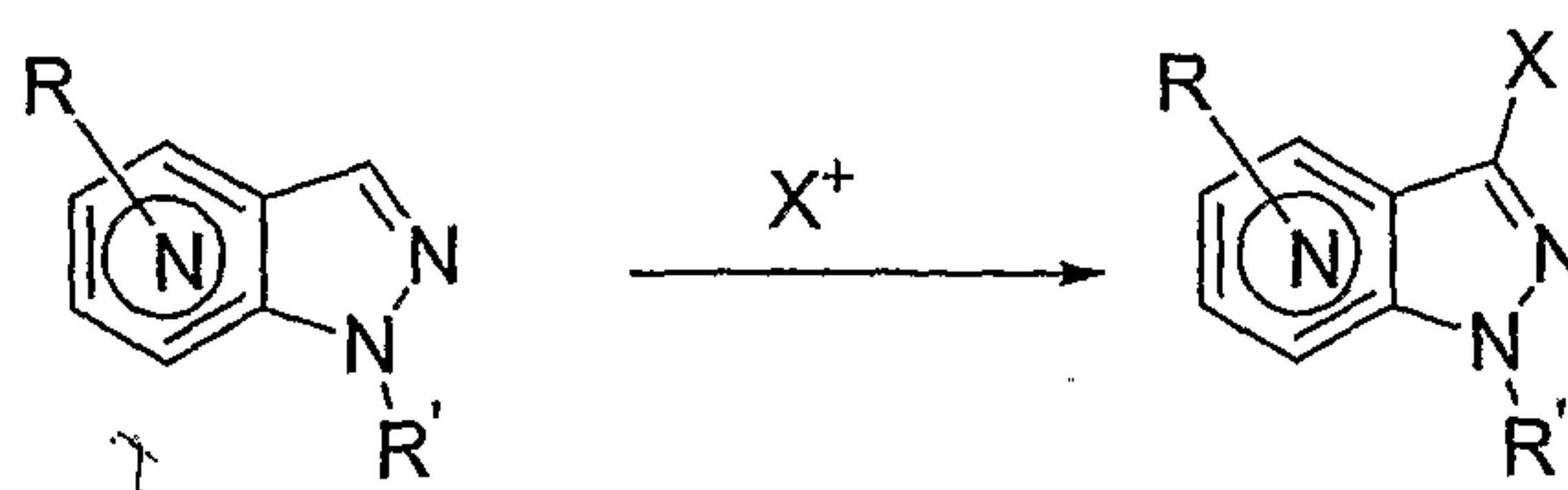
Scheme 1F
