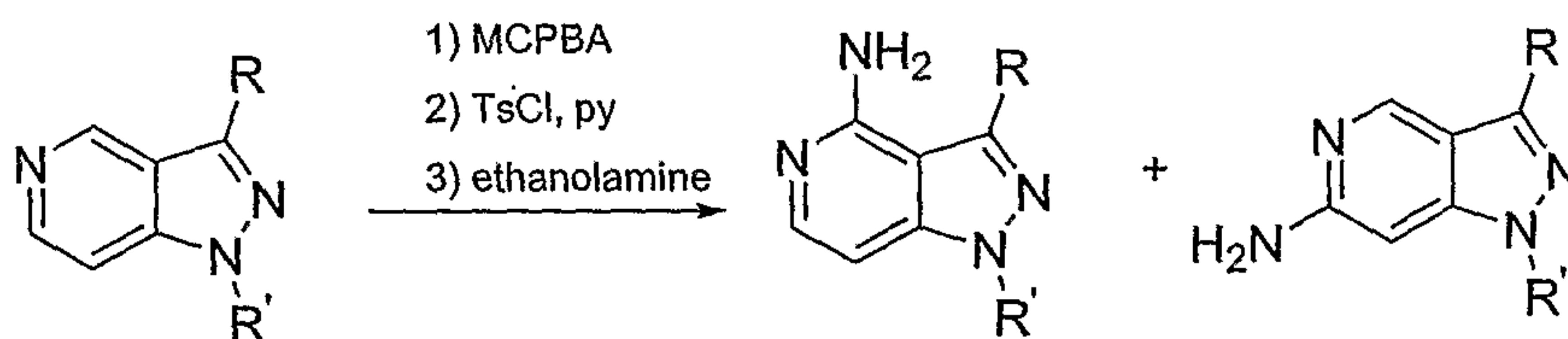
Scheme 1I
