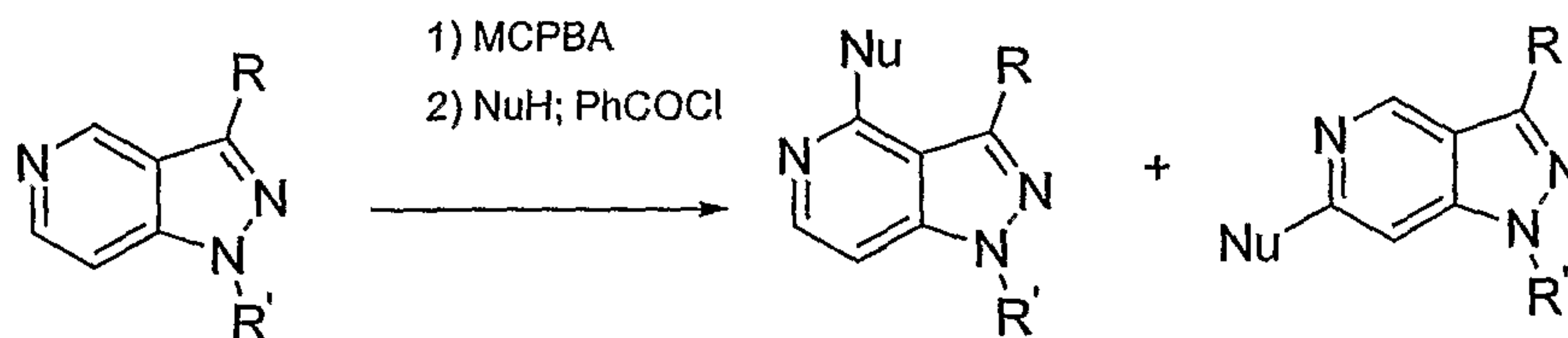
Scheme 1J
