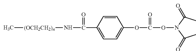
mPEG-Succinimidyl Derivative
