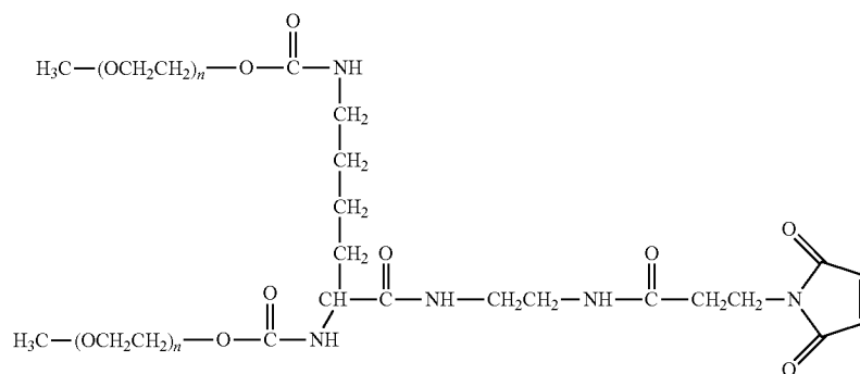
branched mPEG2 Maleimide Derivative
