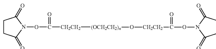
Homobifunctional PEG-Succinimidyl Propionate
