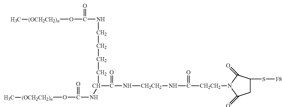
Thioether Linkage
