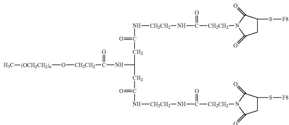
Thioether Linkage
