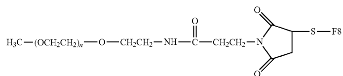
Thioether Linkage
