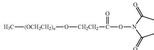
mPEG-Succinimidyl Propionate
