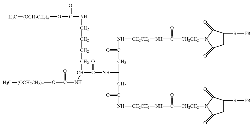
Thioether Linkages
