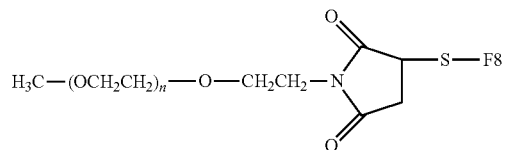
Thioether Linkage
