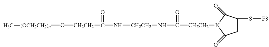
Thioether Linkage
