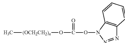
mPEG-Benzotriazole Carbonate
