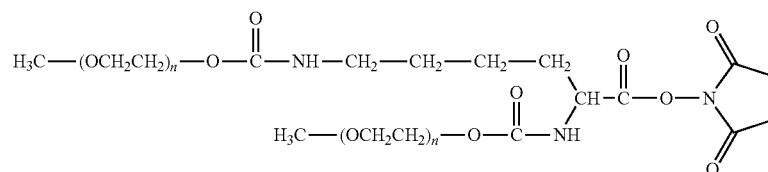
Branched mPEG2-N-Hydroxysuccinimide
