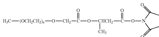
mPEG-Succinimidyl Derivative
