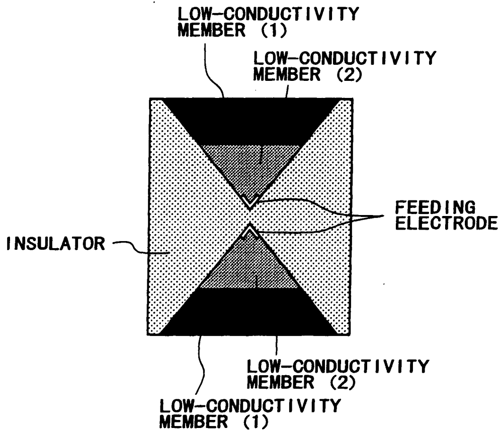
CROSS-SECTIONAL VIEW
