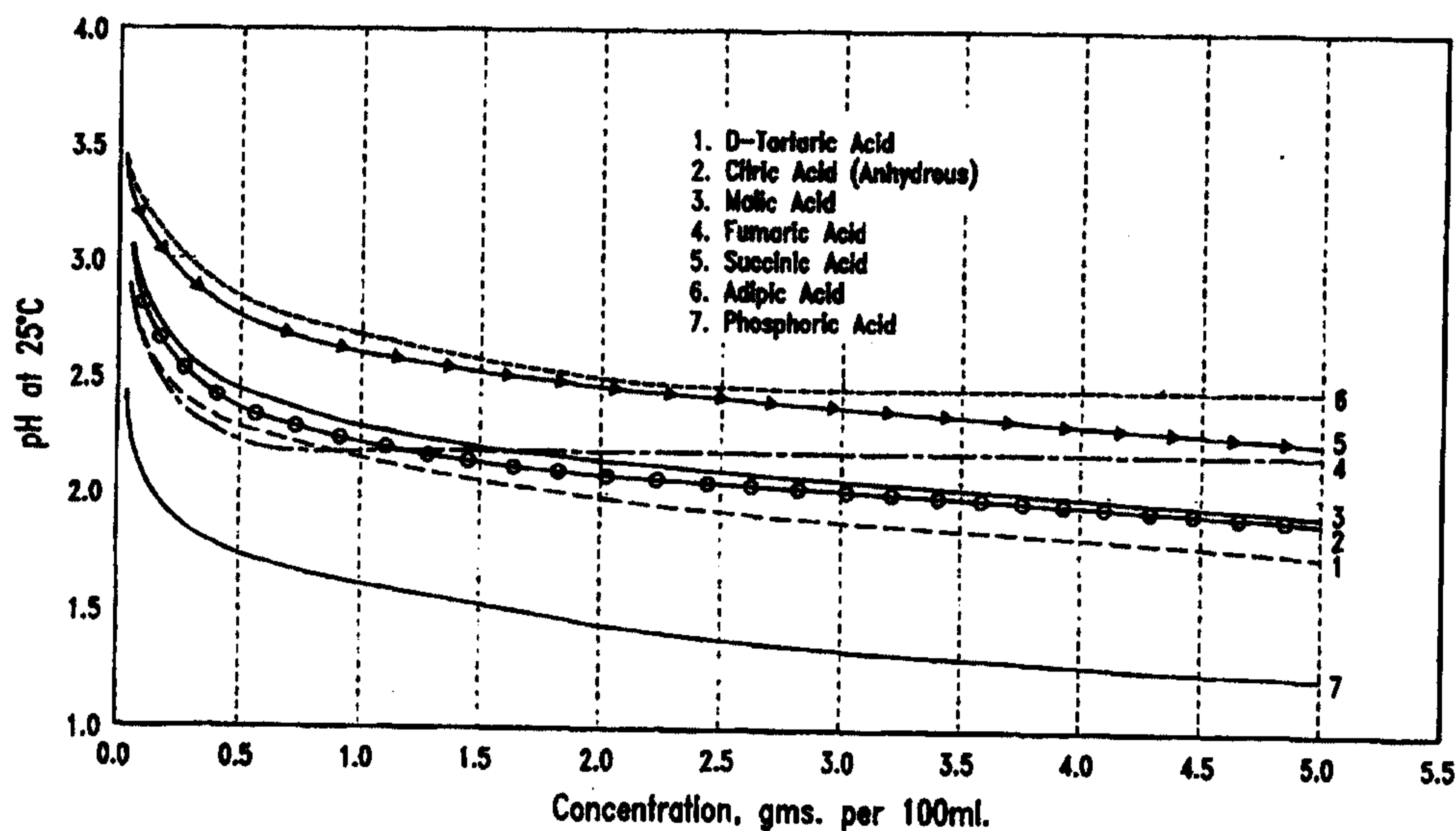
pH of Aqueous Solutions at Various Concentrations.
