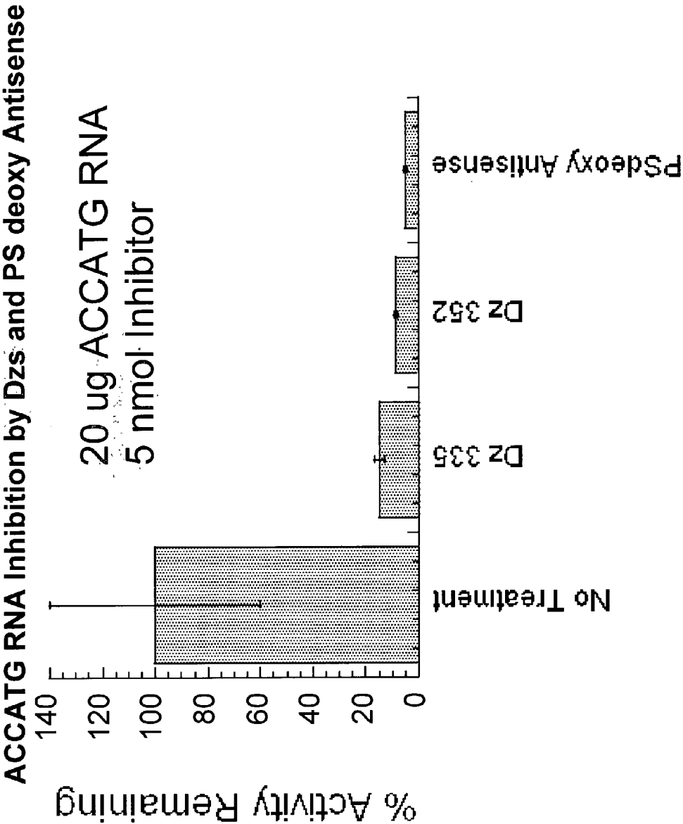
Figure 5B The DNazymes Dz 335 and Dz 352 as well as the antisense molecule Pseodeoxy inhibit translation of ACCATG RNA (same as ACC RNA) by binding to the HCV IRES
