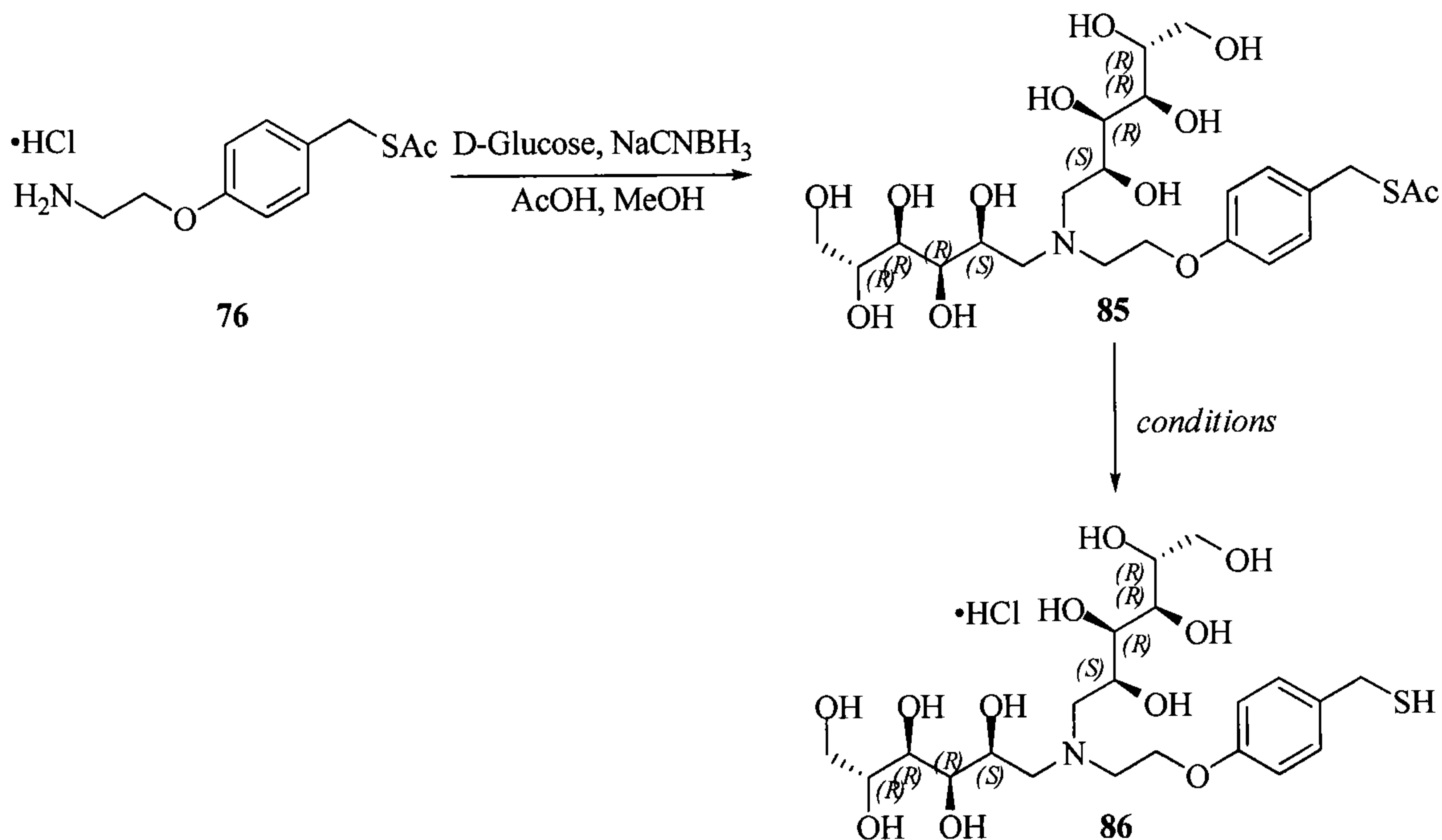
Scheme 22
