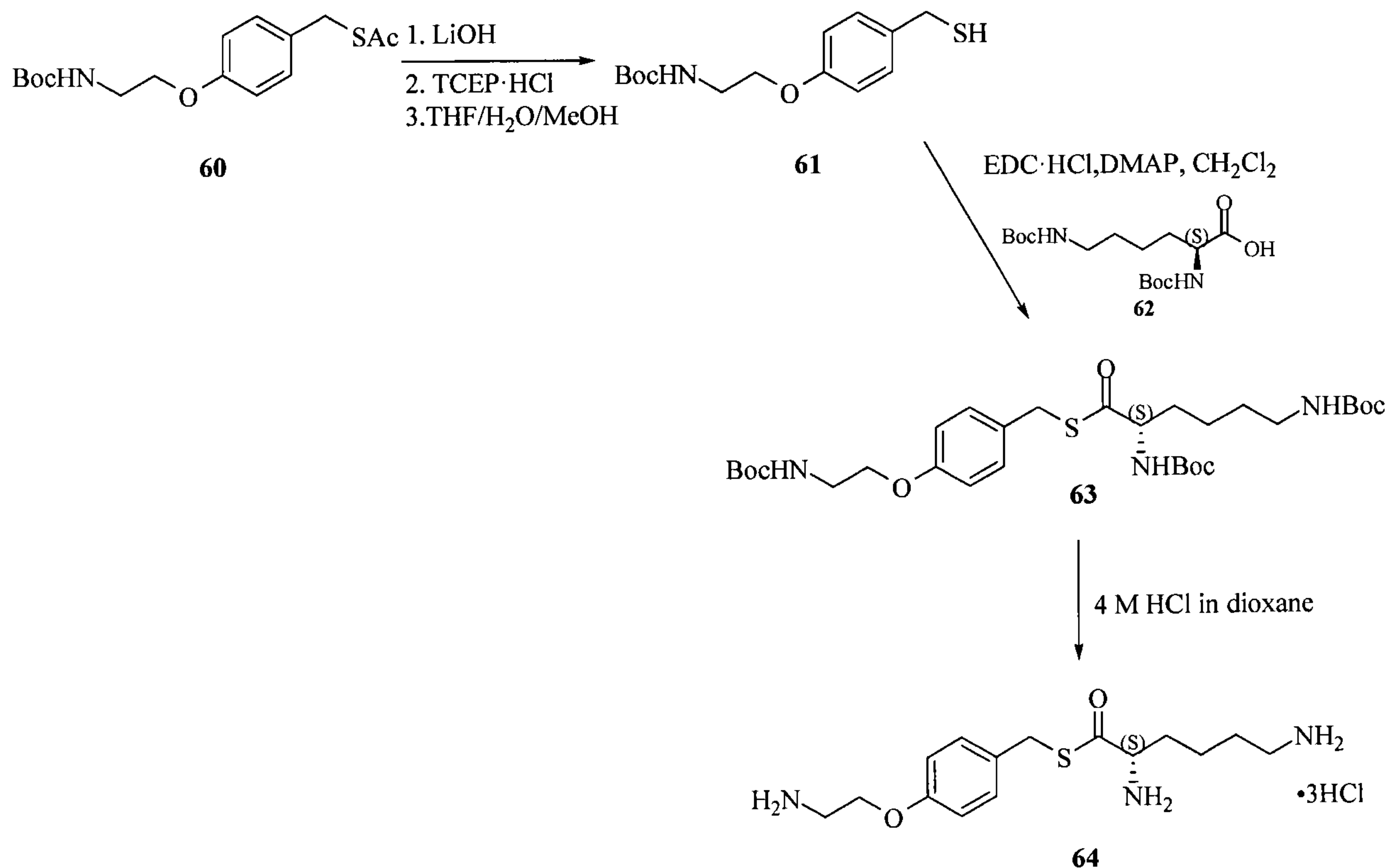
Scheme 15
