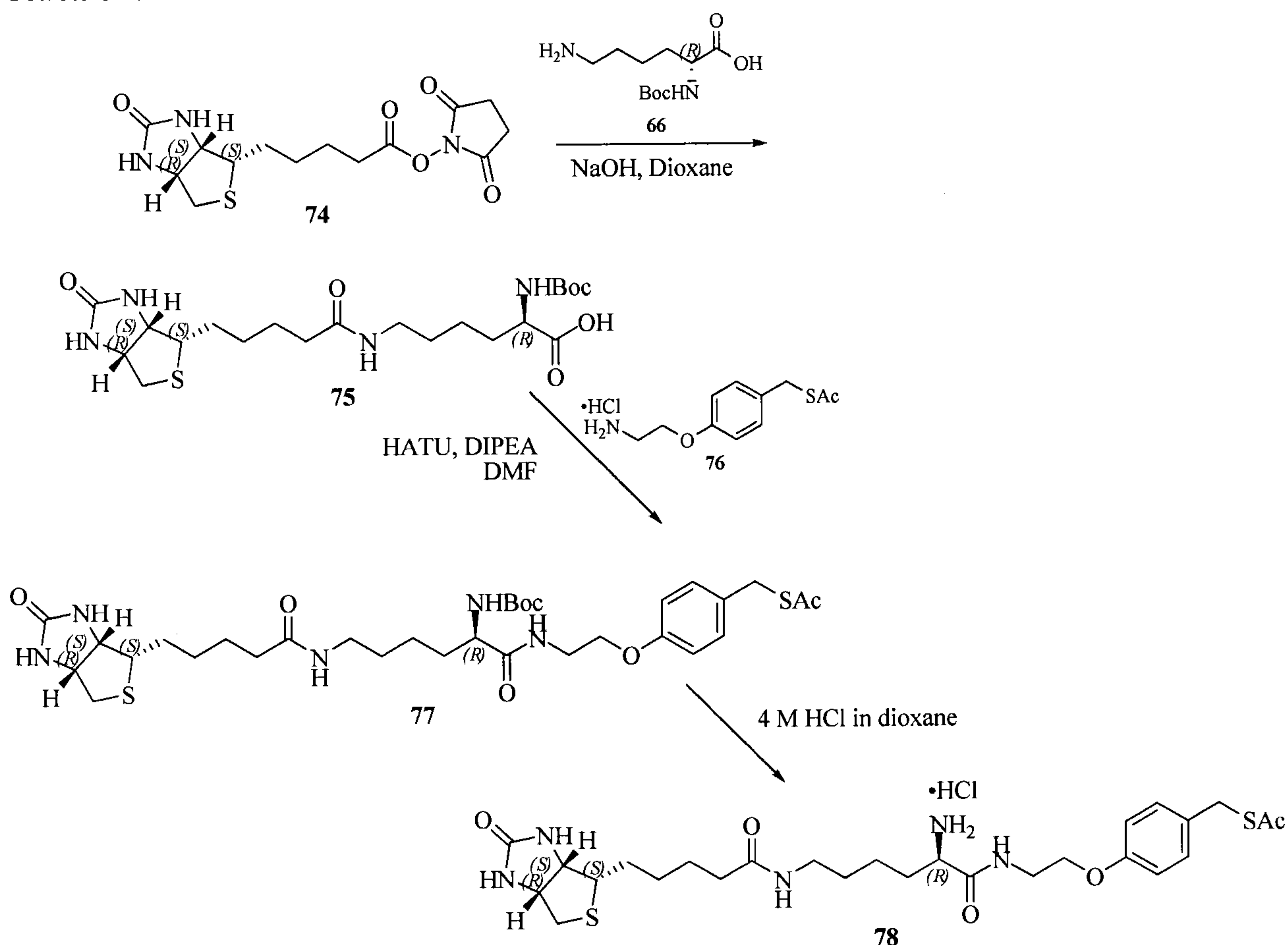
Scheme 19
