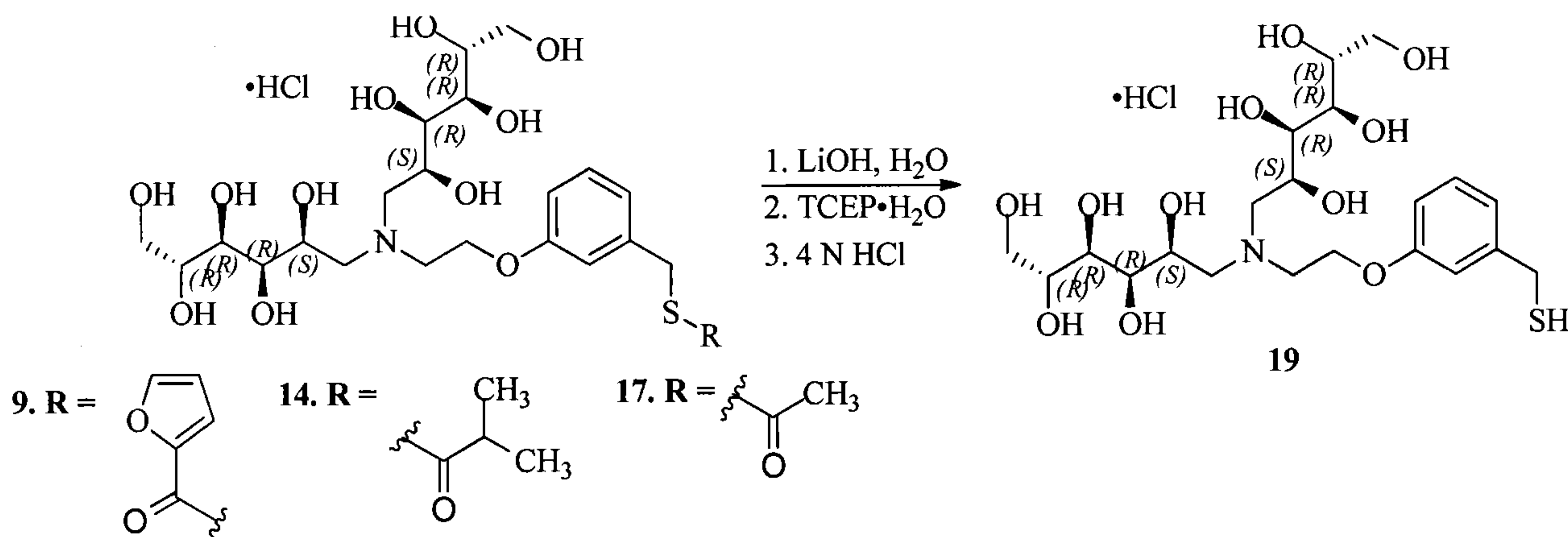
Scheme 7
