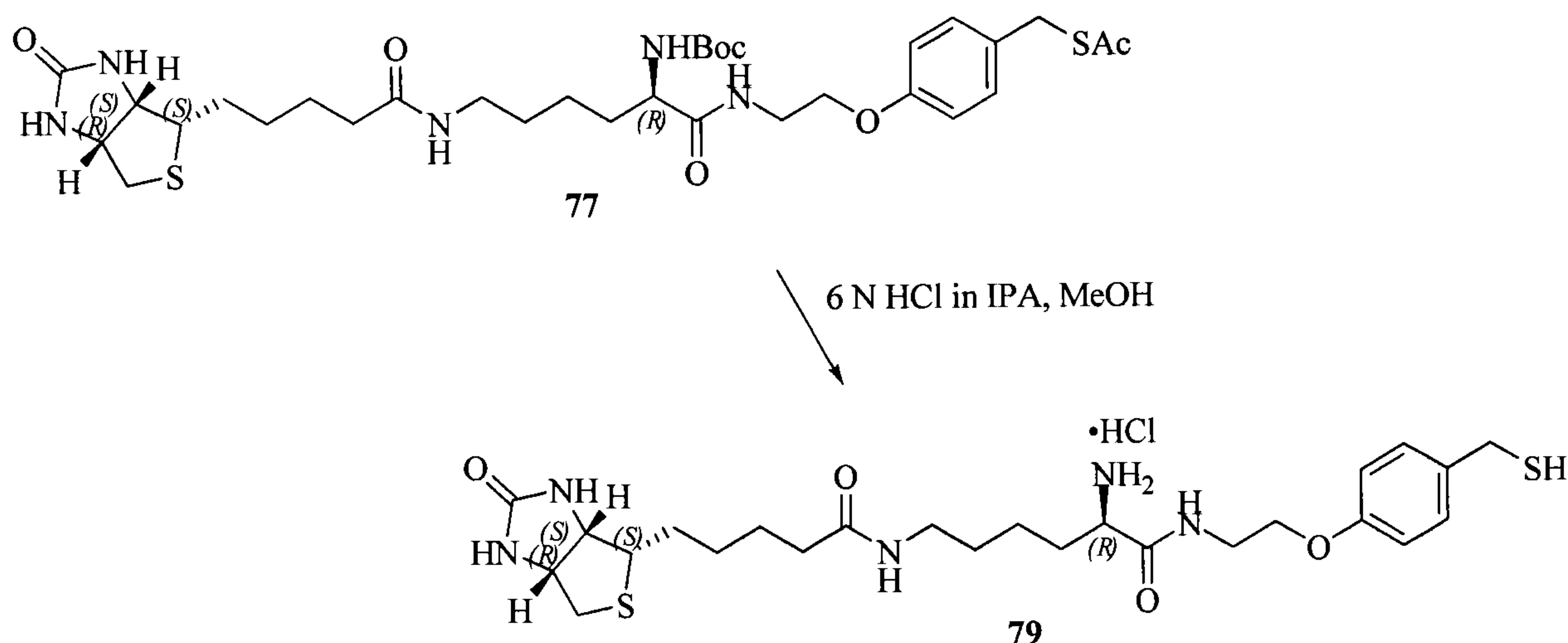
Scheme 20
