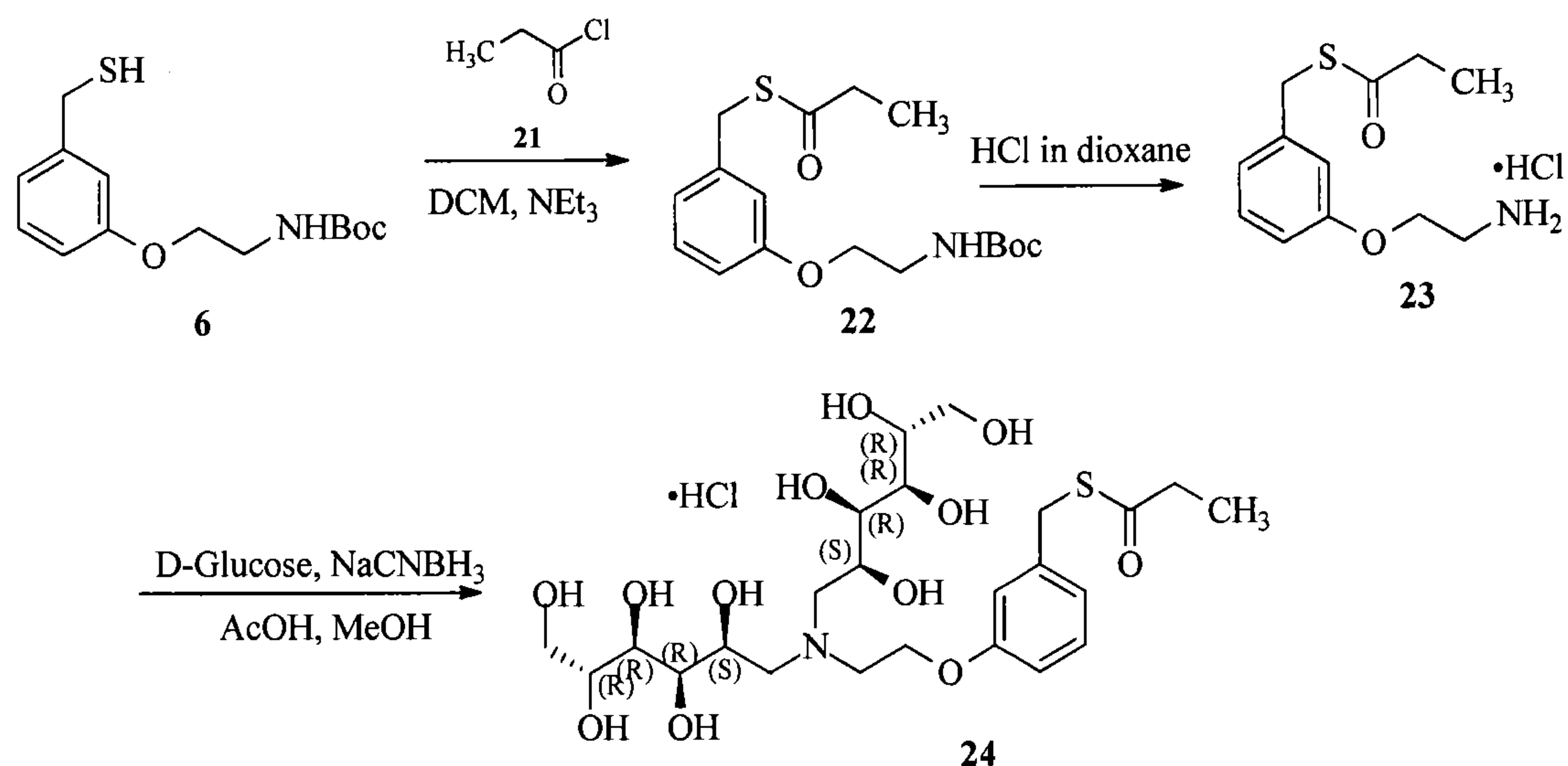
Scheme 9
