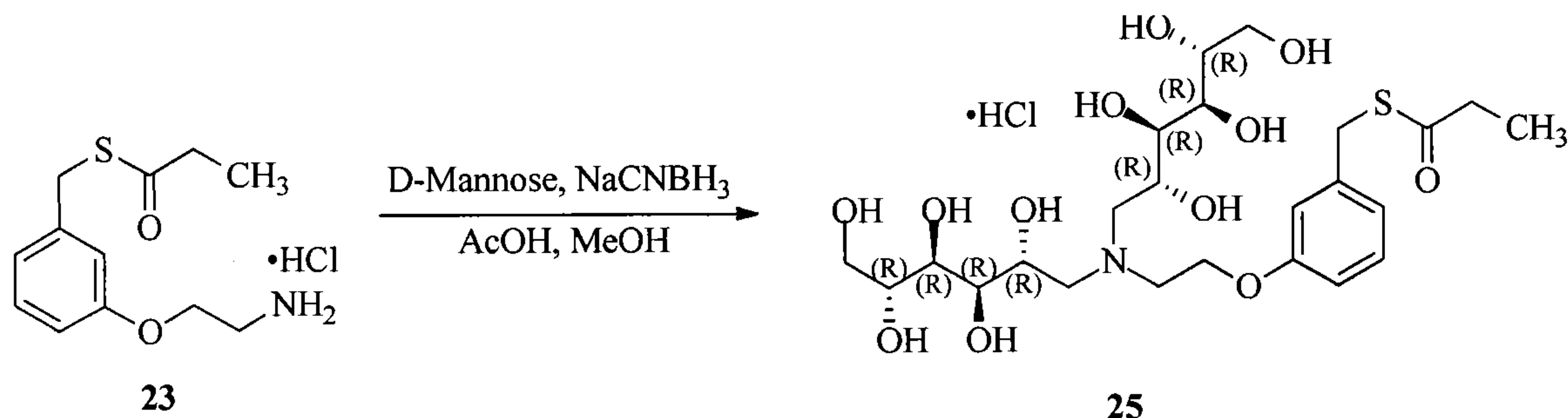
Scheme 10
