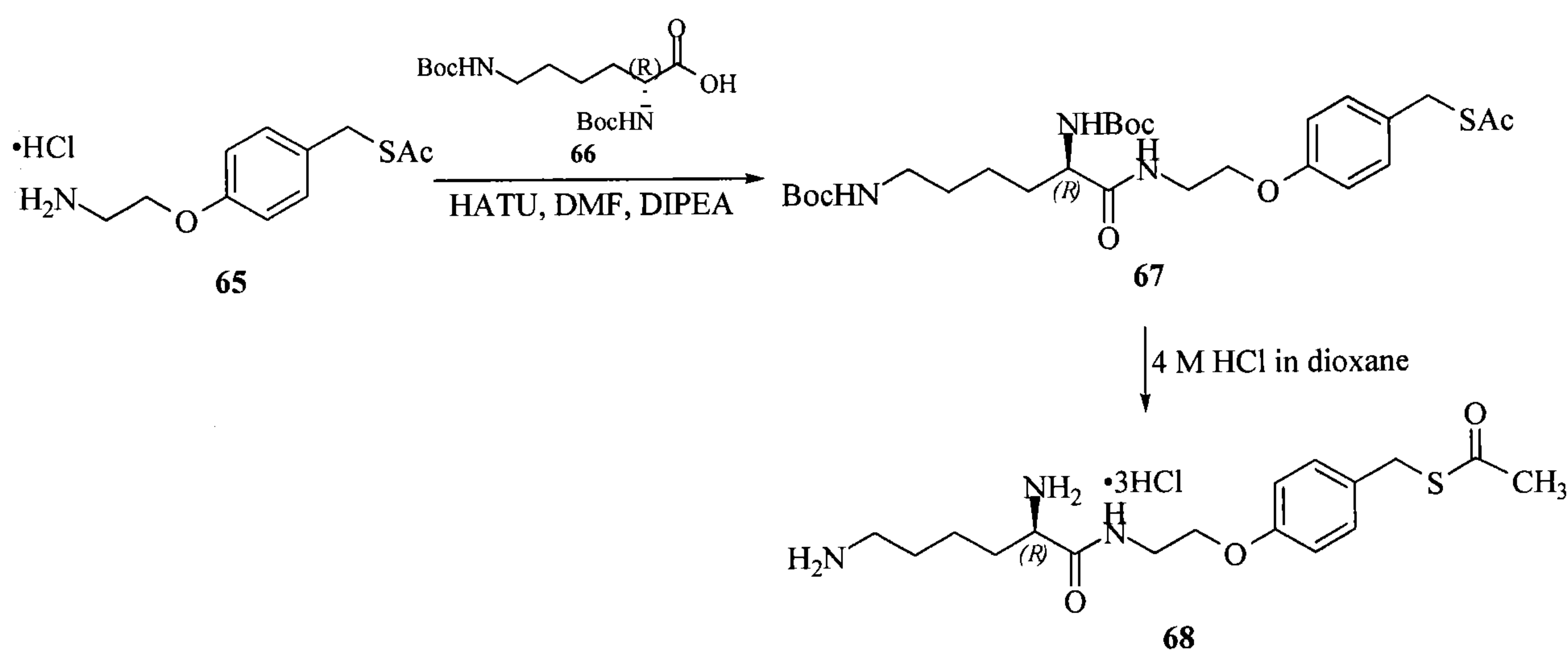
Scheme 16
